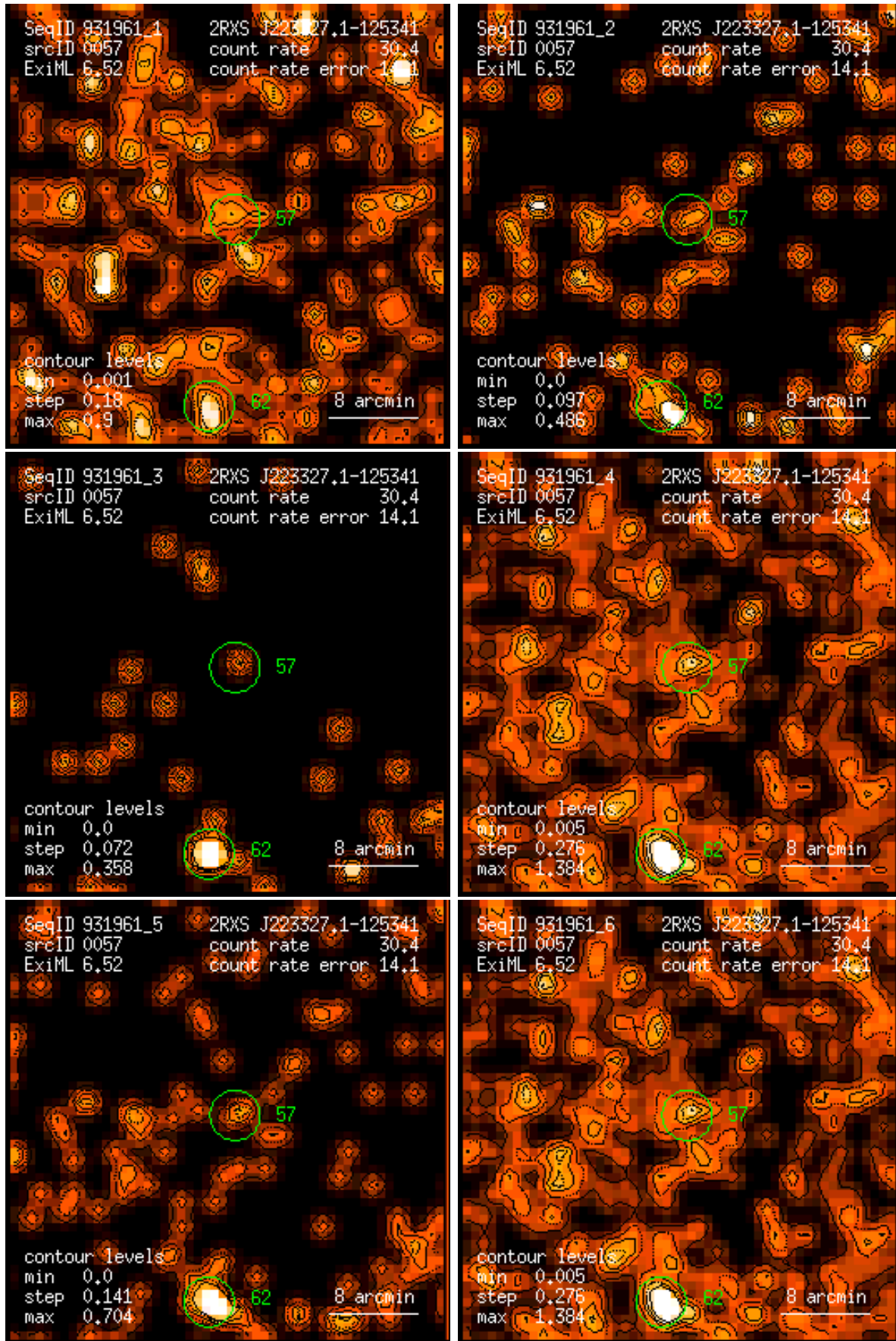
Figure 57: RASS 931961: detection 0057: band rate images, Gaussian filter: (1) PSPC channels 11 – 41, (2) 52 – 90, (3) 91 – 201, (4) 11 – 235, (5) 52 – 201, (6) 11 – 201. Broad band rates in counts/ks. Band rate contour levels in counts/ks/arcmin 2 .
