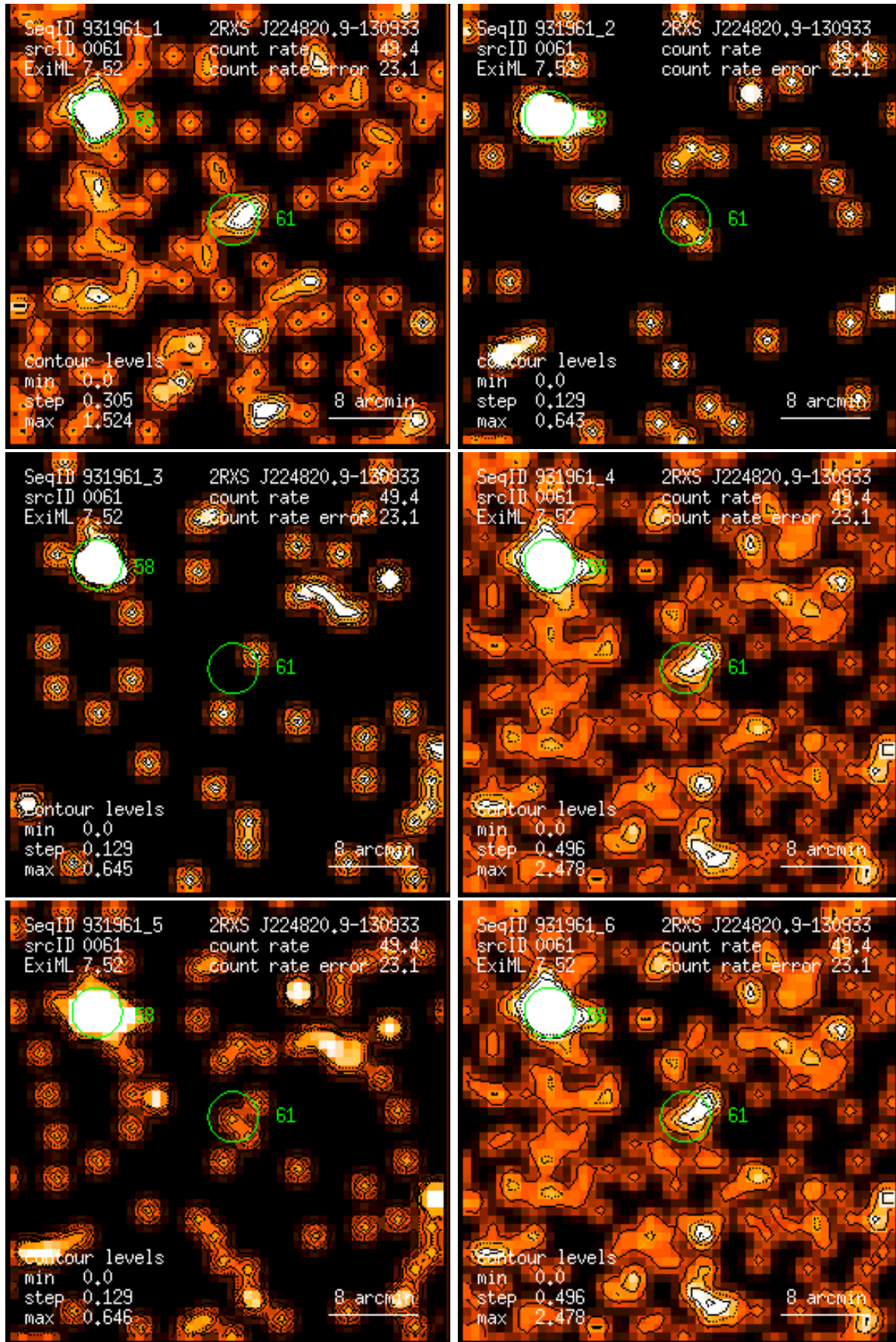
Figure 61: RASS 931961: detection 0061: band rate images, Gaussian filter: (1) PSPC channels 11 – 41, (2) 52 – 90, (3) 91 – 201, (4) 11 – 235, (5) 52 – 201, (6) 11 – 201. Broad band rates in counts/ks. Band rate contour levels in counts/ks/arcmin 2 .
