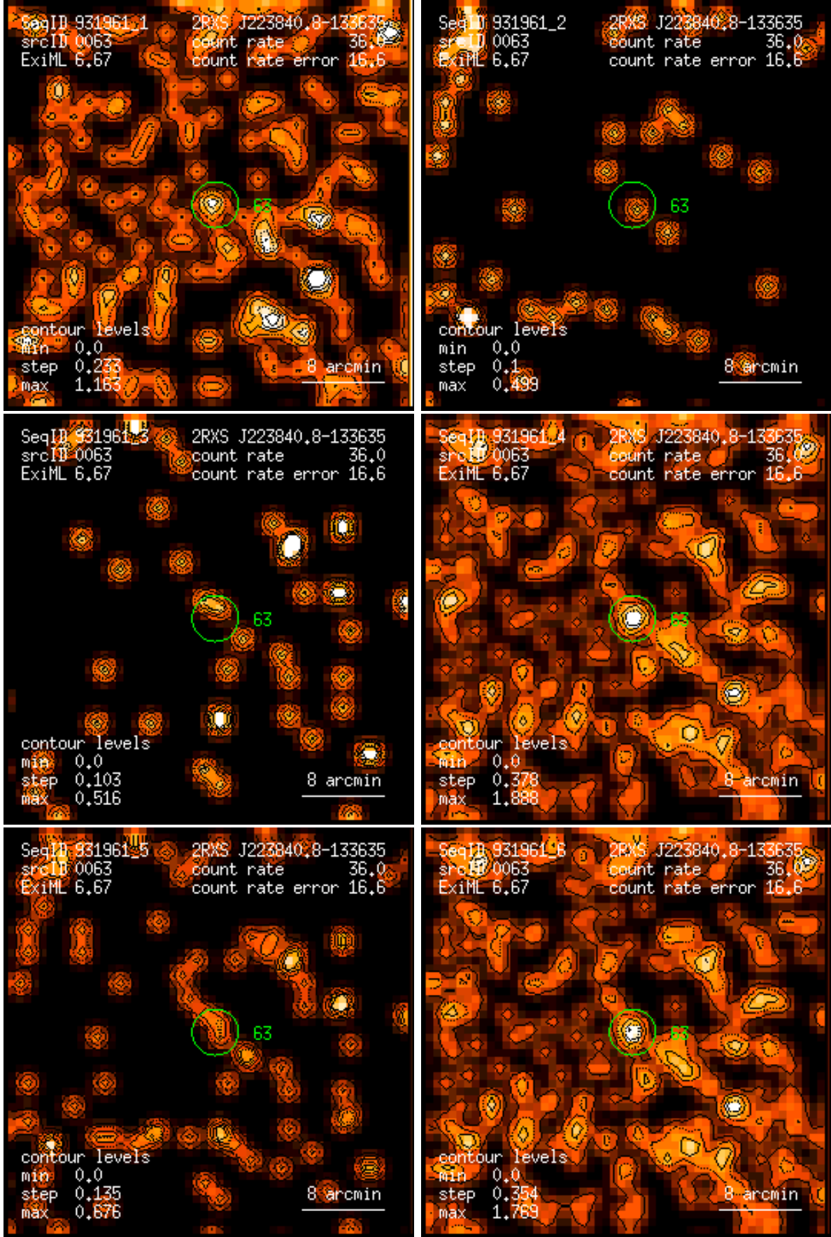
Figure 63: RASS 931961: detection 0063: band rate images, Gaussian filter: (1) PSPC channels 11 – 41, (2) 52 – 90, (3) 91 – 201, (4) 11 – 235, (5) 52 – 201, (6) 11 – 201. Broad band rates in counts/ks. Band rate contour levels in counts/ks/arcmin 2 .
