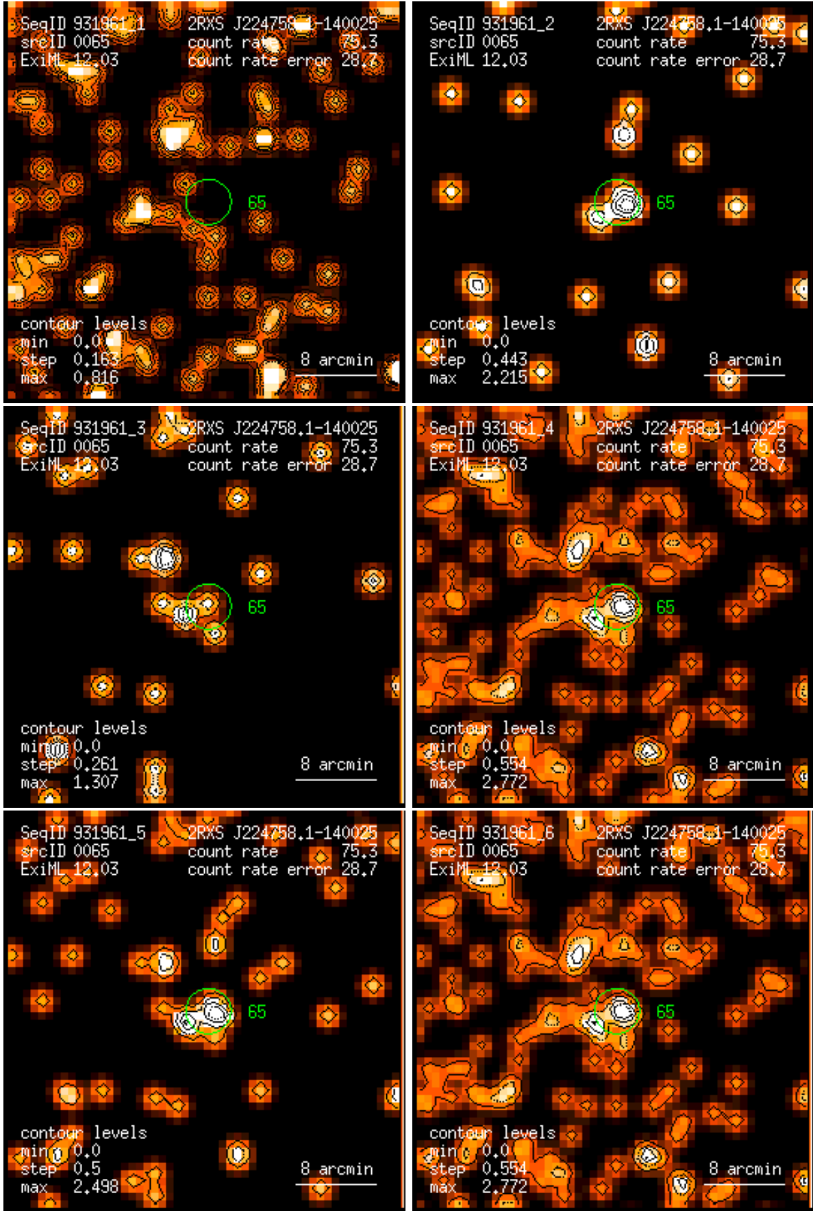
Figure 65: RASS 931961: detection 0065: band rate images, Gaussian filter: (1) PSPC channels 11 – 41, (2) 52 – 90, (3) 91 – 201, (4) 11 – 235, (5) 52 – 201, (6) 11 – 201. Broad band rates in counts/ks. Band rate contour levels in counts/ks/arcmin 2 .
