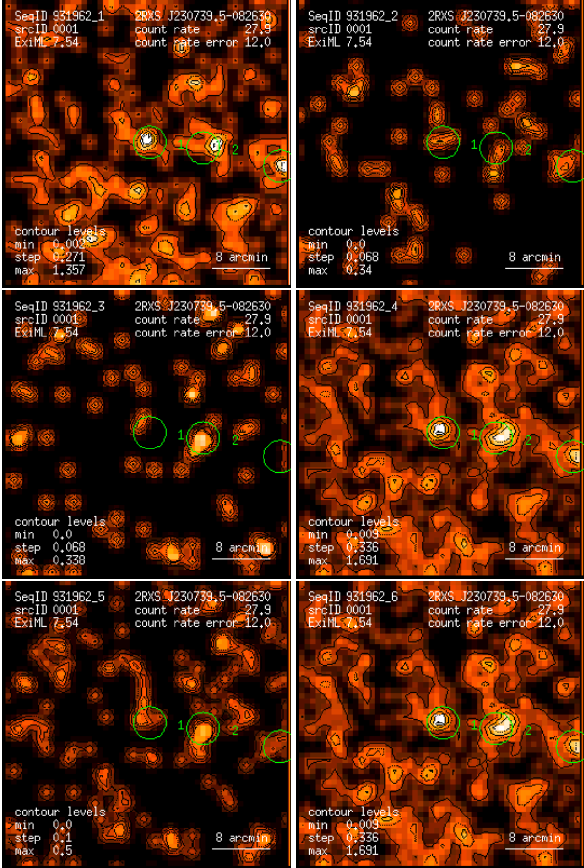
Figure 1: RASS 931962: detection 0001: band rate images, Gaussian filter: (1) PSPC channels 11 – 41, (2) 52 – 90, (3) 91 – 201, (4) 11 – 235, (5) 52 – 201, (6) 11 – 201. Broad band rates in counts/ks. Band rate contour levels in counts/ks/arcmin 2 .
