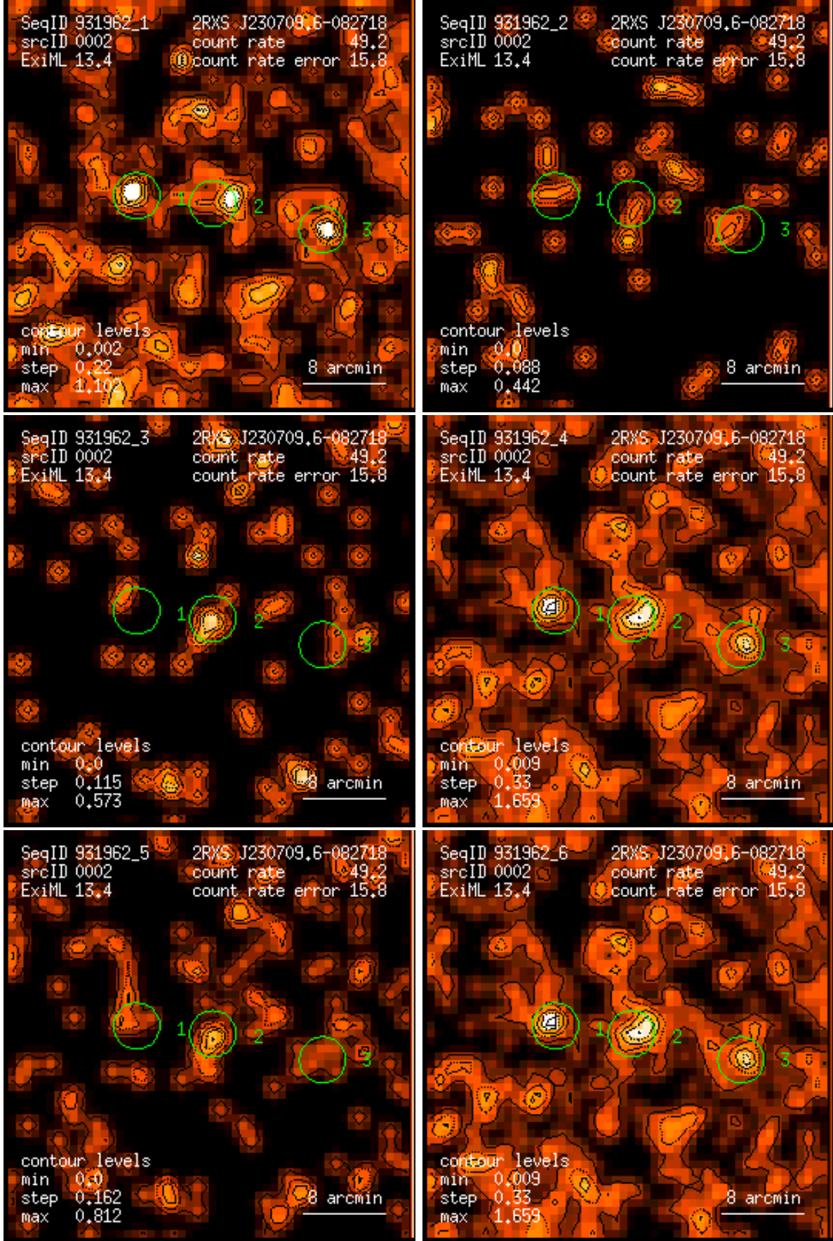
Figure 2: RASS 931962: detection 0002: band rate images, Gaussian filter: (1) PSPC channels 11 – 41, (2) 52 – 90, (3) 91 – 201, (4) 11 – 235, (5) 52 – 201, (6) 11 – 201. Broad band rates in counts/ks. Band rate contour levels in counts/ks/arcmin 2 .
