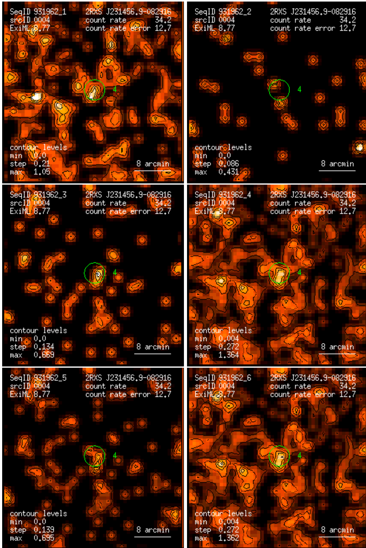
Figure 4: RASS 931962: detection 0004: band rate images, Gaussian filter: (1) PSPC channels 11 – 41, (2) 52 – 90, (3) 91 – 201, (4) 11 – 235, (5) 52 – 201, (6) 11 – 201. Broad band rates in counts/ks. Band rate contour levels in counts/ks/arcmin 2 .
