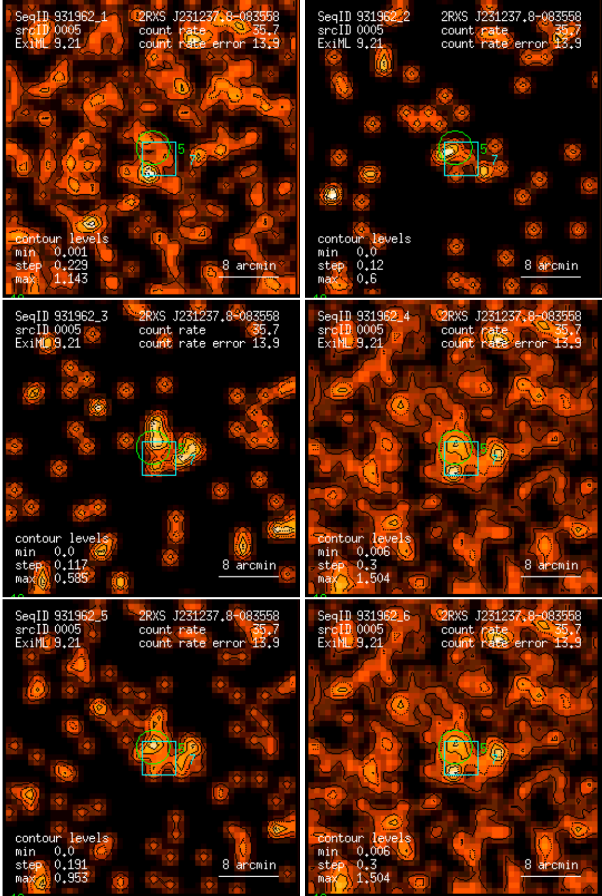
Figure 5: RASS 931962: detection 0005: band rate images, Gaussian filter: (1) PSPC channels 11 – 41, (2) 52 – 90, (3) 91 – 201, (4) 11 – 235, (5) 52 – 201, (6) 11 – 201. Broad band rates in counts/ks. Band rate contour levels in counts/ks/arcmin 2 .
