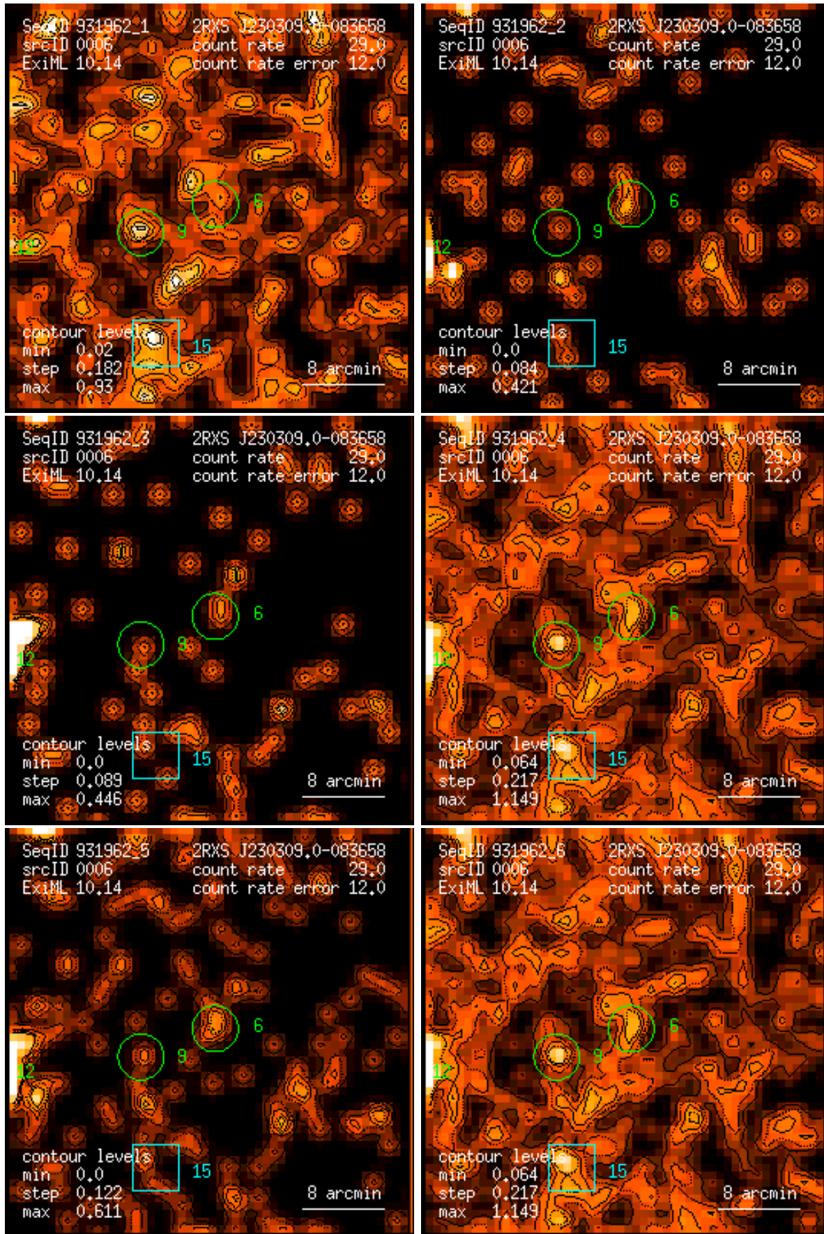
Figure 6: RASS 931962: detection 0006: band rate images, Gaussian filter: (1) PSPC channels 11 – 41, (2) 52 – 90, (3) 91 – 201, (4) 11 – 235, (5) 52 – 201, (6) 11 – 201. Broad band rates in counts/ks. Band rate contour levels in counts/ks/arcmin 2 .
