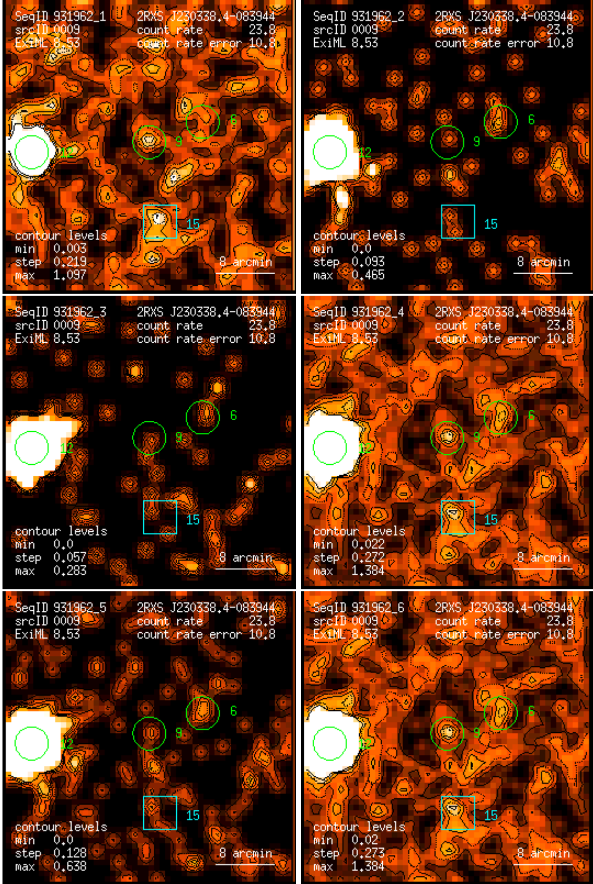
Figure 9: RASS 931962: detection 0009: band rate images, Gaussian filter: (1) PSPC channels 11 – 41, (2) 52 – 90, (3) 91 – 201, (4) 11 – 235, (5) 52 – 201, (6) 11 – 201. Broad band rates in counts/ks. Band rate contour levels in counts/ks/arcmin 2 .
