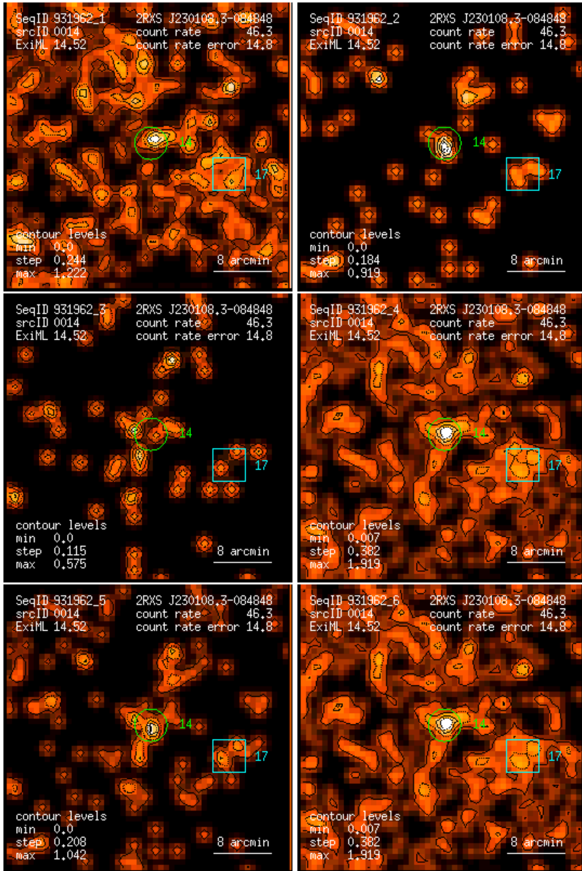
Figure 14: RASS 931962: detection 0014: band rate images, Gaussian filter: (1) PSPC channels 11 – 41, (2) 52 – 90, (3) 91 – 201, (4) 11 – 235, (5) 52 – 201, (6) 11 – 201. Broad band rates in counts/ks. Band rate contour levels in counts/ks/arcmin 2 .
