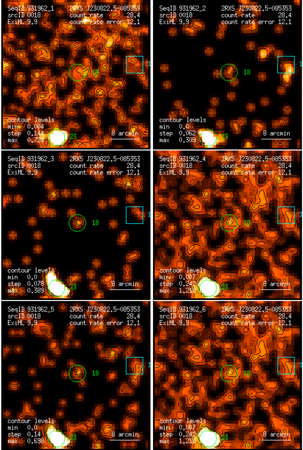
Figure 18: RASS 931962: detection 0018: band rate images, Gaussian filter: (1) PSPC channels 11 – 41, (2) 52 – 90, (3) 91 – 201, (4) 11 – 235, (5) 52 – 201, (6) 11 – 201. Broad band rates in counts/ks. Band rate contour levels in counts/ks/arcmin 2 .
