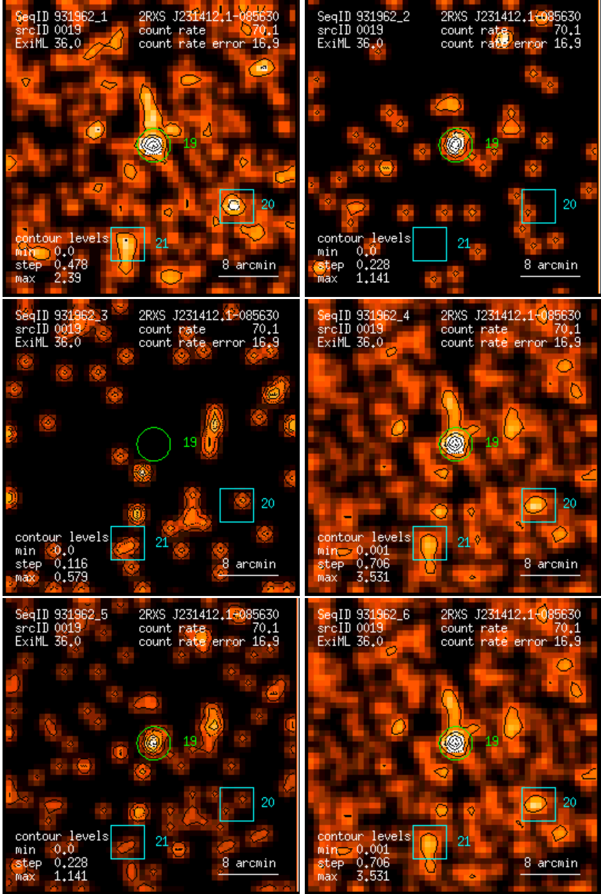
Figure 19: RASS 931962: detection 0019: band rate images, Gaussian filter: (1) PSPC channels 11 – 41, (2) 52 – 90, (3) 91 – 201, (4) 11 – 235, (5) 52 – 201, (6) 11 – 201. Broad band rates in counts/ks. Band rate contour levels in counts/ks/arcmin 2 .
