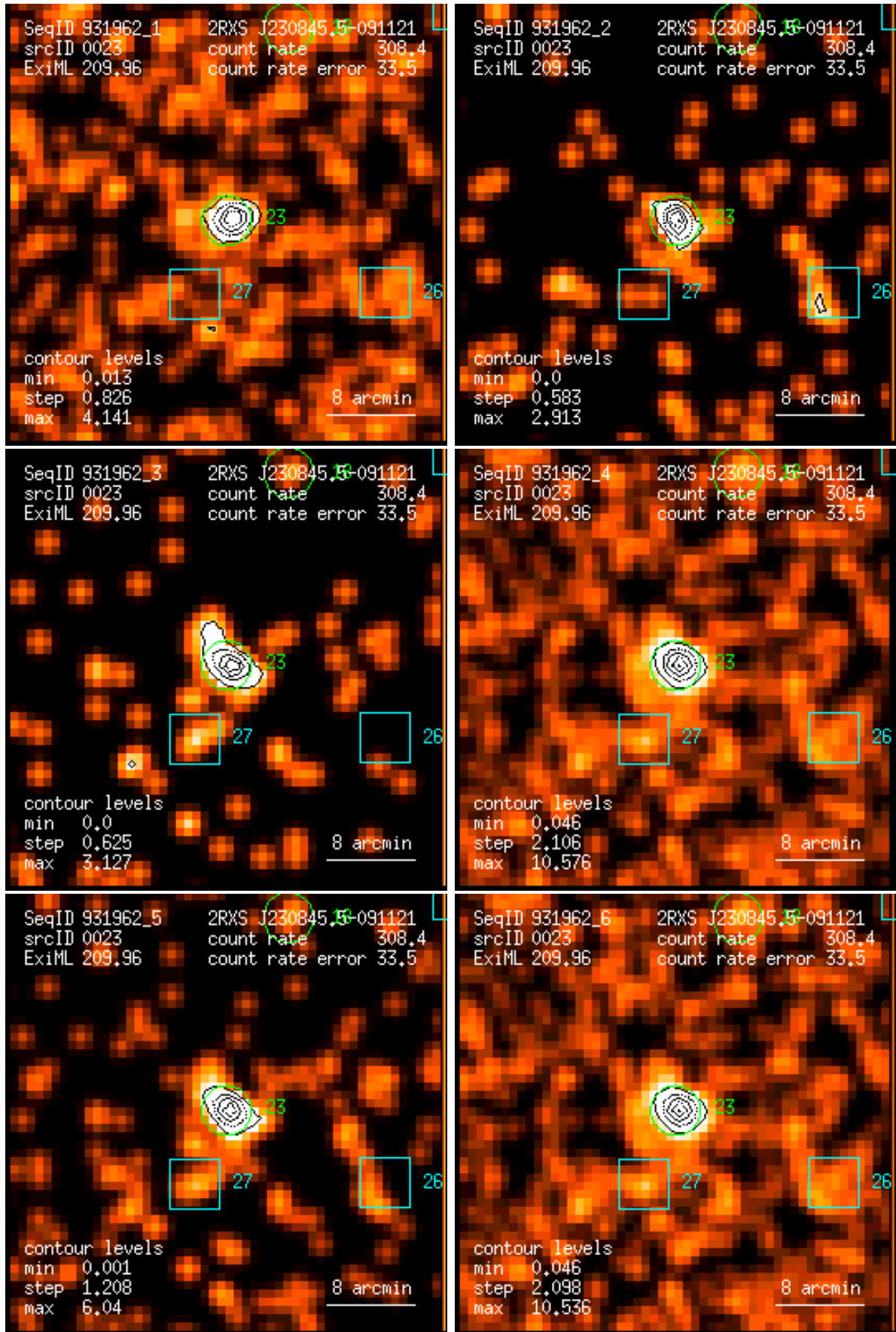
Figure 23: RASS 931962: detection 0023: band rate images, Gaussian filter: (1) PSPC channels 11 – 41, (2) 52 – 90, (3) 91 – 201, (4) 11 – 235, (5) 52 – 201, (6) 11 – 201. Broad band rates in counts/ks. Band rate contour levels in counts/ks/arcmin 2 .
