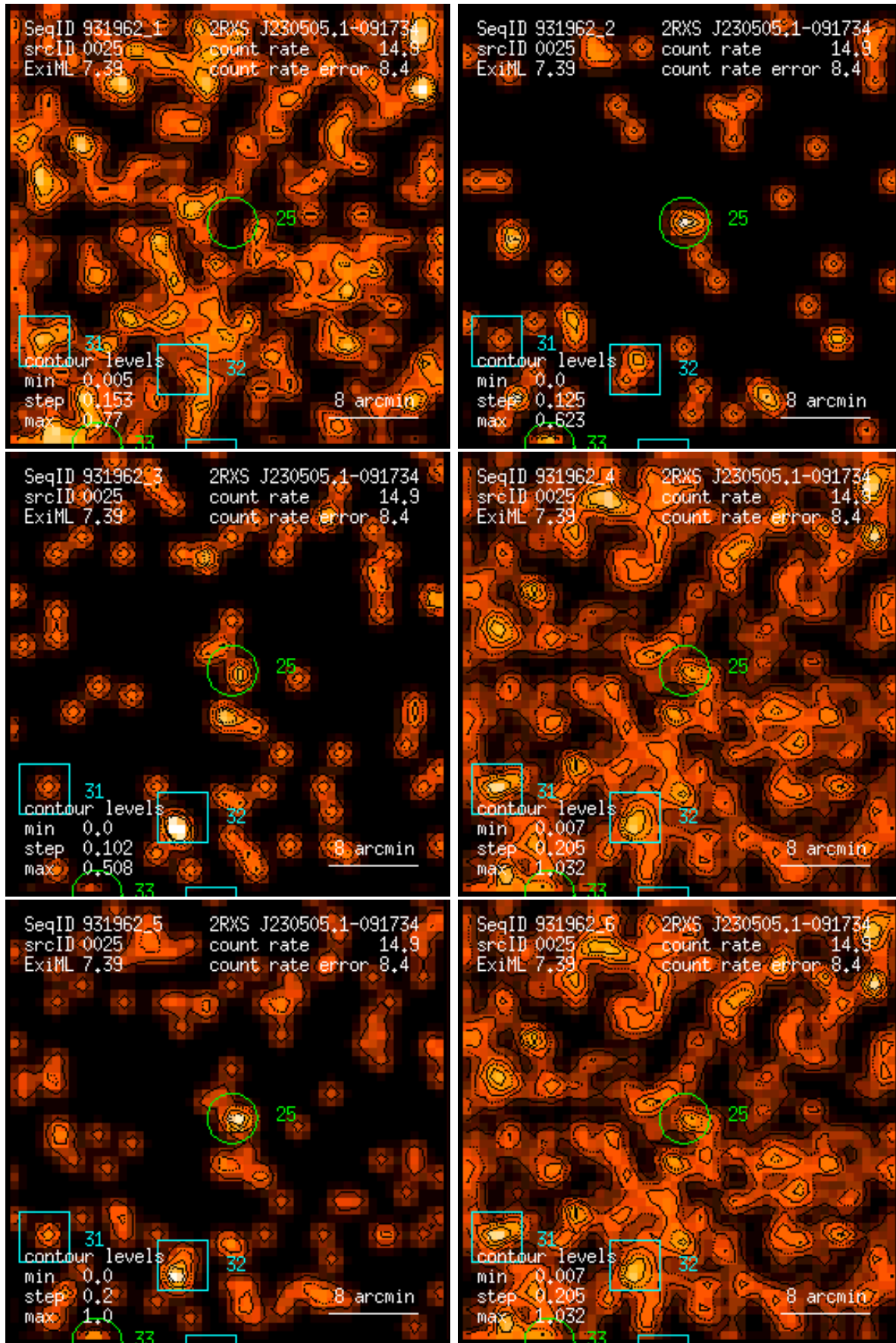
Figure 25: RASS 931962: detection 0025: band rate images, Gaussian filter: (1) PSPC channels 11 – 41, (2) 52 – 90, (3) 91 – 201, (4) 11 – 235, (5) 52 – 201, (6) 11 – 201. Broad band rates in counts/ks. Band rate contour levels in counts/ks/arcmin 2 .
