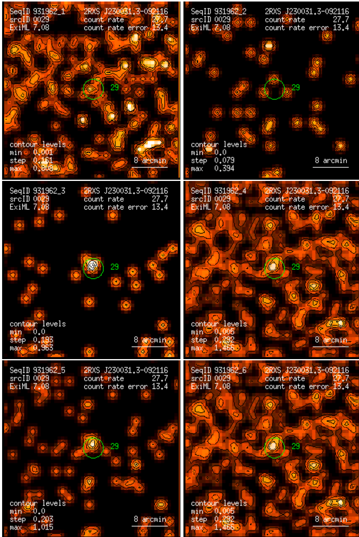
Figure 29: RASS 931962: detection 0029: band rate images, Gaussian filter: (1) PSPC channels 11 – 41, (2) 52 – 90, (3) 91 – 201, (4) 11 – 235, (5) 52 – 201, (6) 11 – 201. Broad band rates in counts/ks. Band rate contour levels in counts/ks/arcmin 2 .
