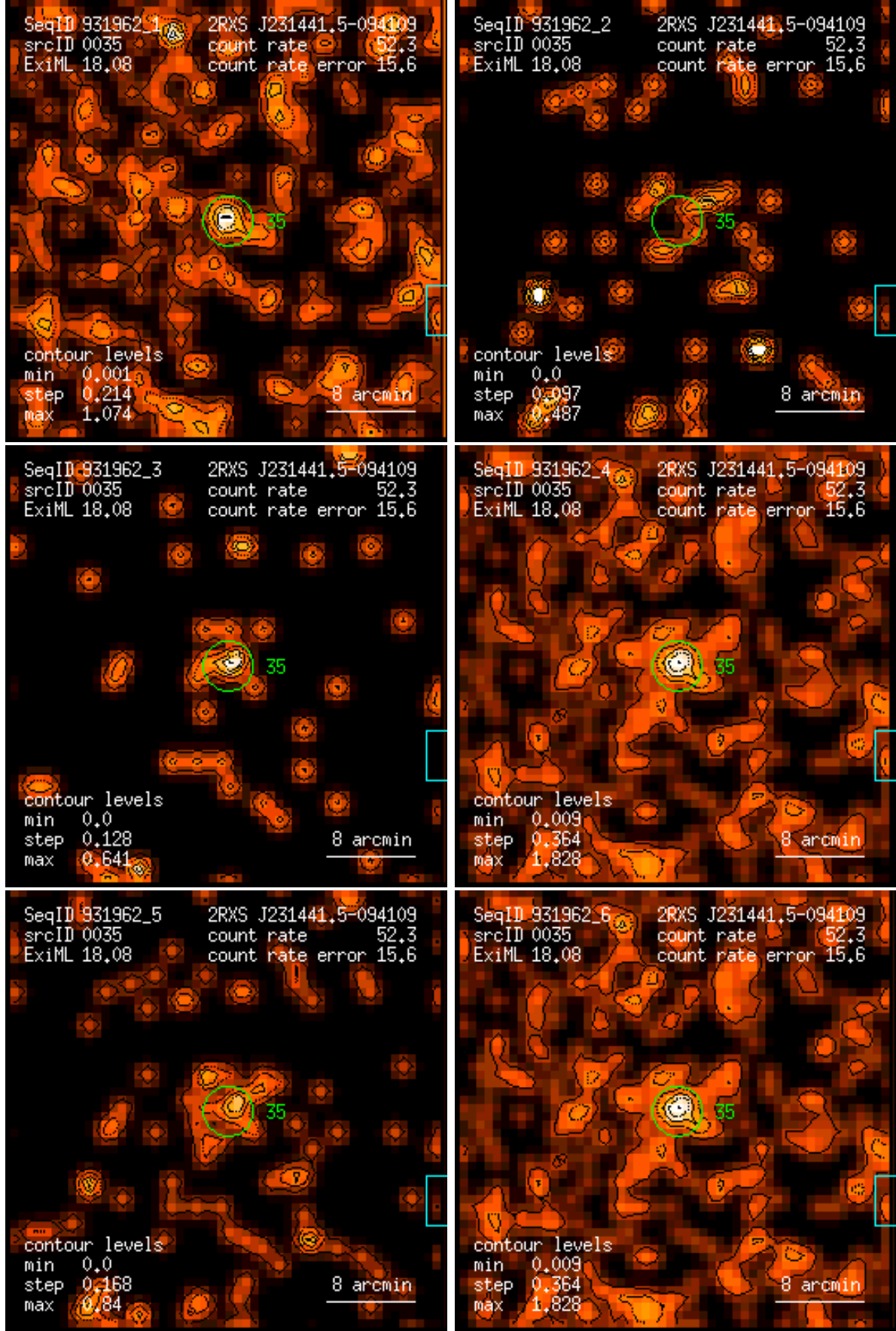
Figure 35: RASS 931962: detection 0035: band rate images, Gaussian filter: (1) PSPC channels 11 – 41, (2) 52 – 90, (3) 91 – 201, (4) 11 – 235, (5) 52 – 201, (6) 11 – 201. Broad band rates in counts/ks. Band rate contour levels in counts/ks/arcmin 2 .
