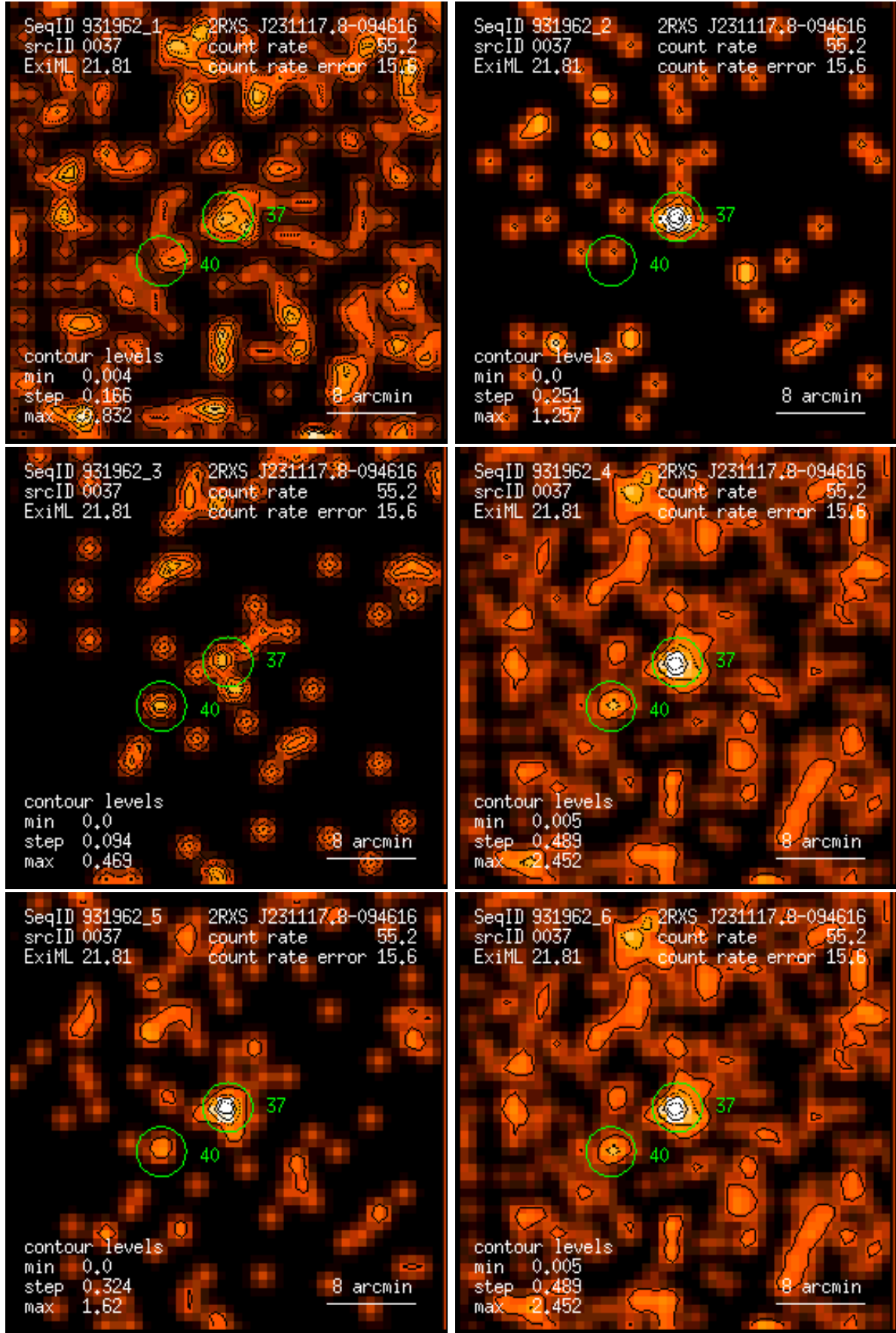
Figure 37: RASS 931962: detection 0037: band rate images, Gaussian filter: (1) PSPC channels 11 – 41, (2) 52 – 90, (3) 91 – 201, (4) 11 – 235, (5) 52 – 201, (6) 11 – 201. Broad band rates in counts/ks. Band rate contour levels in counts/ks/arcmin 2 .
