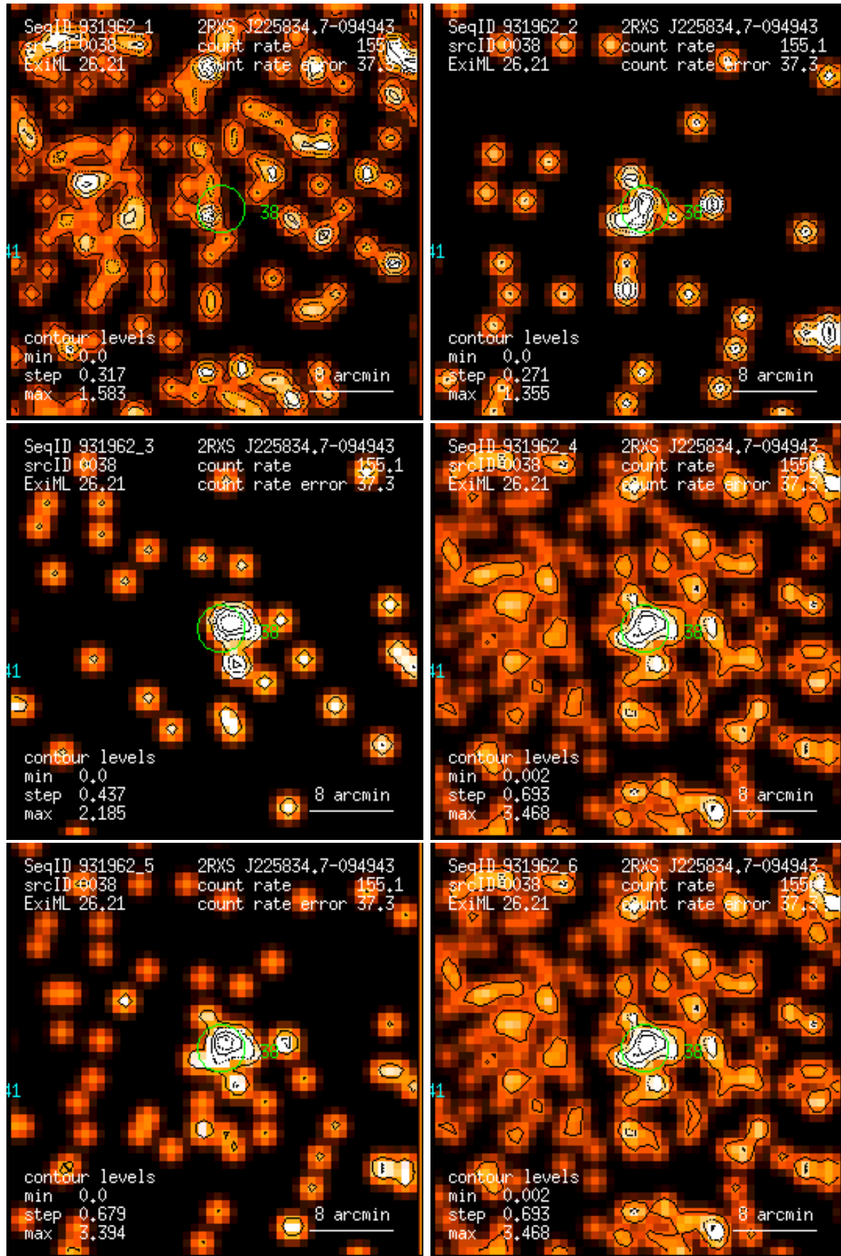
Figure 38: RASS 931962: detection 0038: band rate images, Gaussian filter: (1) PSPC channels 11 – 41, (2) 52 – 90, (3) 91 – 201, (4) 11 – 235, (5) 52 – 201, (6) 11 – 201. Broad band rates in counts/ks. Band rate contour levels in counts/ks/arcmin 2 .
