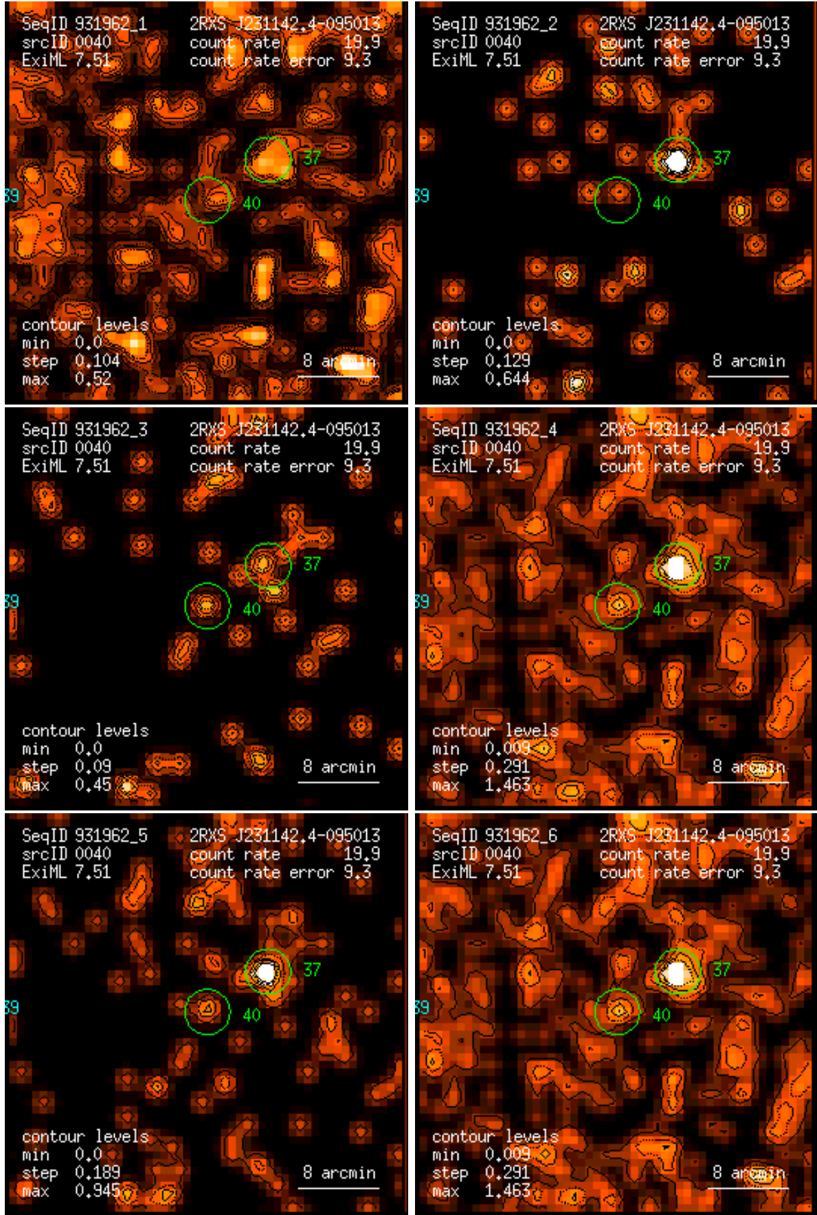
Figure 40: RASS 931962: detection 0040: band rate images, Gaussian filter: (1) PSPC channels 11 – 41, (2) 52 – 90, (3) 91 – 201, (4) 11 – 235, (5) 52 – 201, (6) 11 – 201. Broad band rates in counts/ks. Band rate contour levels in counts/ks/arcmin 2 .
