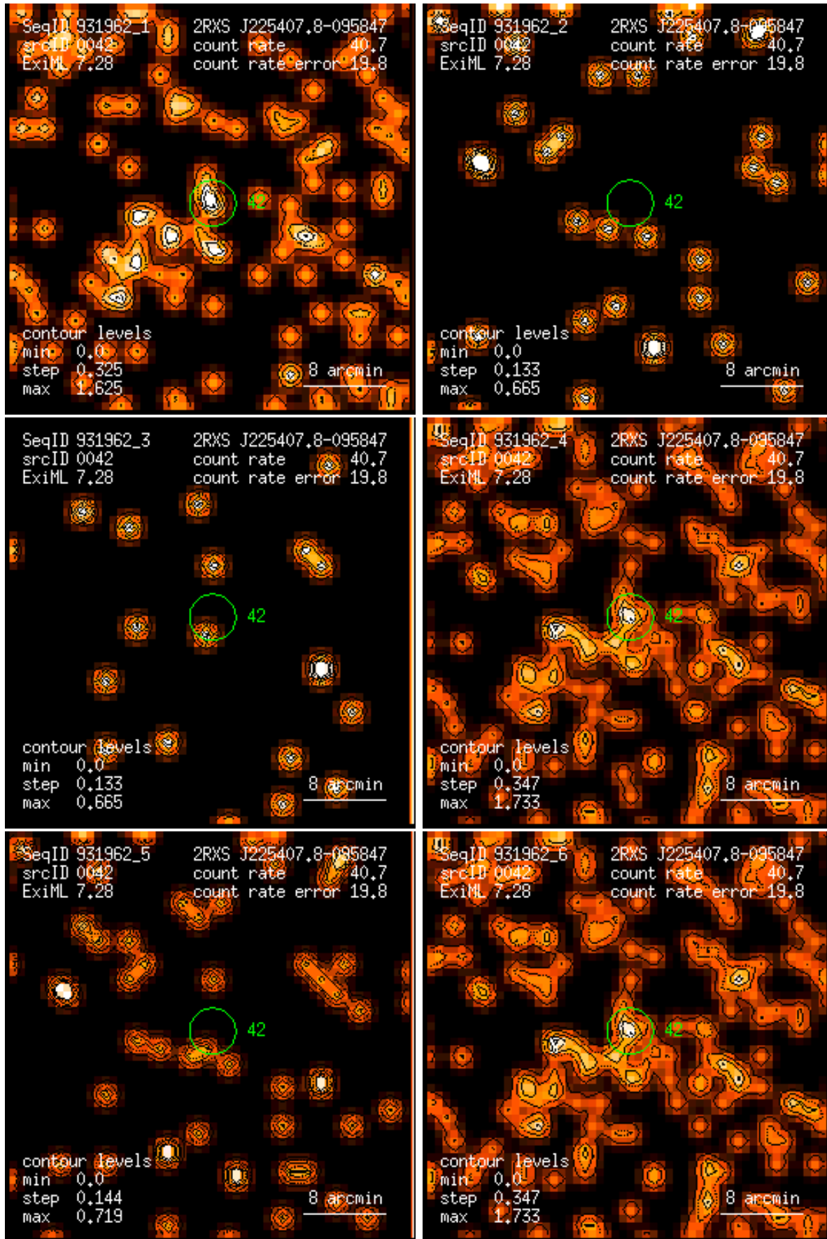
Figure 42: RASS 931962: detection 0042: band rate images, Gaussian filter: (1) PSPC channels 11 – 41, (2) 52 – 90, (3) 91 – 201, (4) 11 – 235, (5) 52 – 201, (6) 11 – 201. Broad band rates in counts/ks. Band rate contour levels in counts/ks/arcmin 2 .
