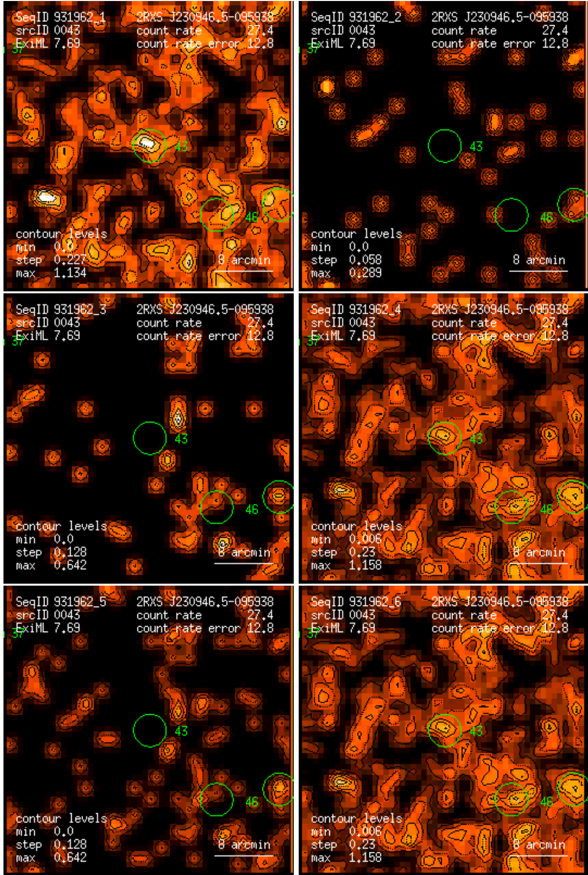
Figure 43: RASS 931962: detection 0043: band rate images, Gaussian filter: (1) PSPC channels 11 – 41, (2) 52 – 90, (3) 91 – 201, (4) 11 – 235, (5) 52 – 201, (6) 11 – 201. Broad band rates in counts/ks. Band rate contour levels in counts/ks/arcmin 2 .
