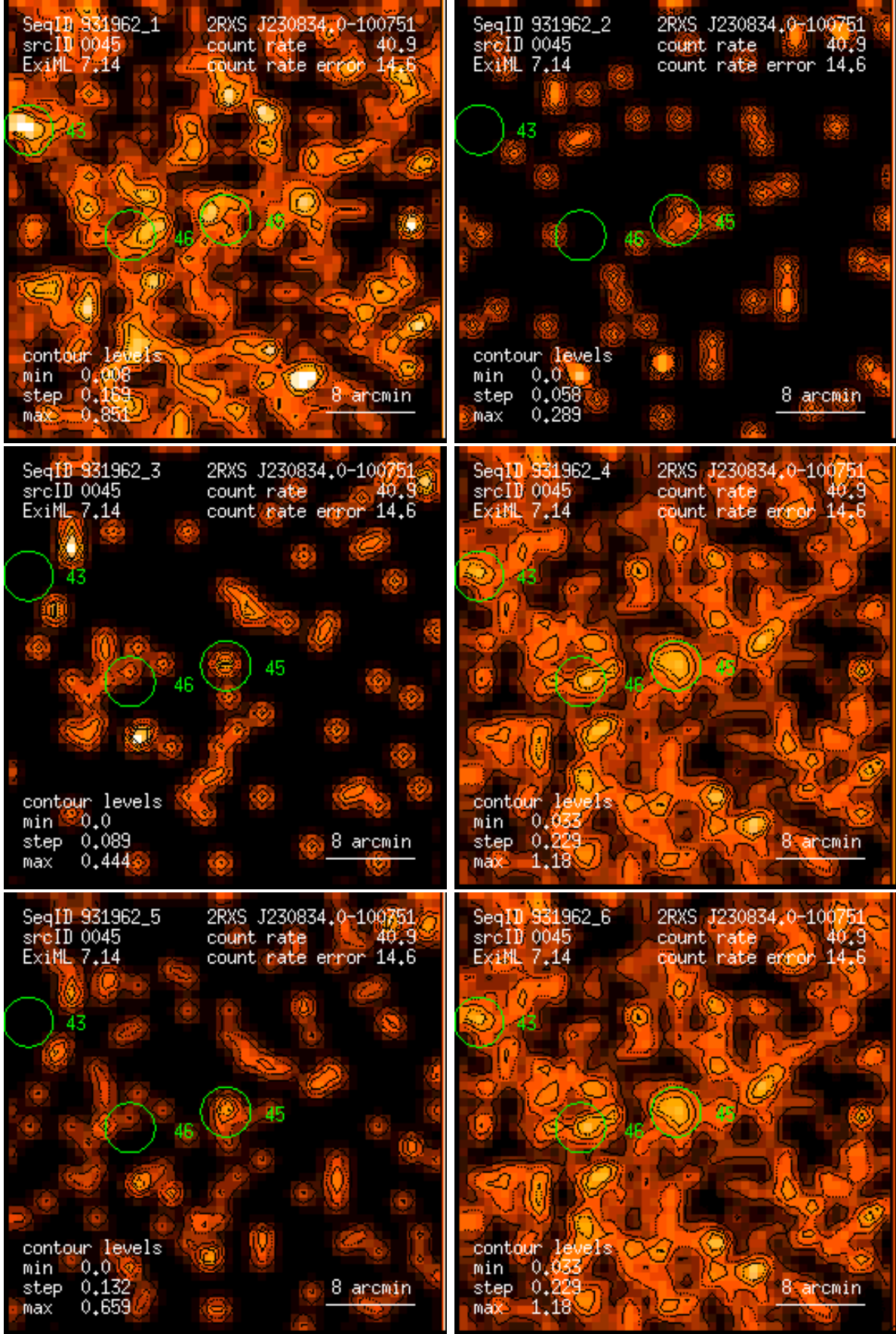
Figure 45: RASS 931962: detection 0045: band rate images, Gaussian filter: (1) PSPC channels 11 – 41, (2) 52 – 90, (3) 91 – 201, (4) 11 – 235, (5) 52 – 201, (6) 11 – 201. Broad band rates in counts/ks. Band rate contour levels in counts/ks/arcmin 2 .
