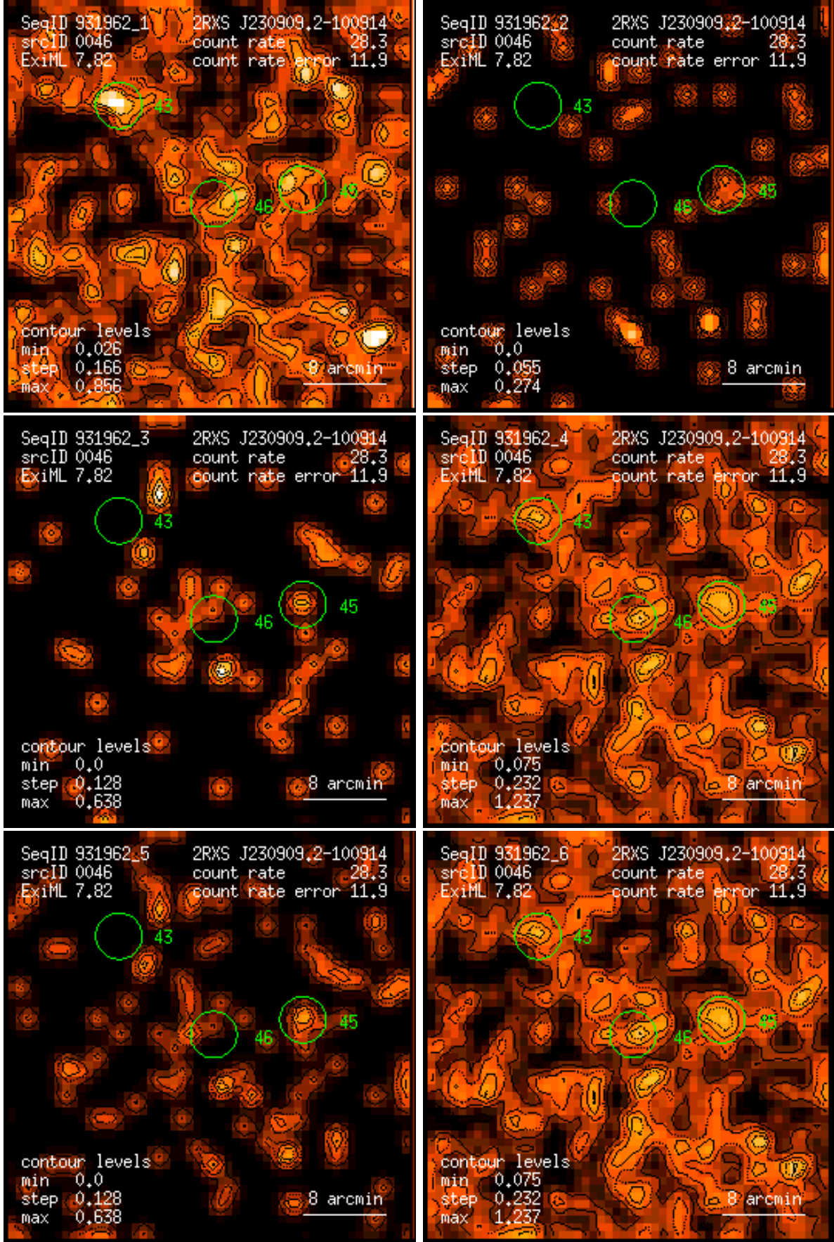
Figure 46: RASS 931962: detection 0046: band rate images, Gaussian filter: (1) PSPC channels 11 – 41, (2) 52 – 90, (3) 91 – 201, (4) 11 – 235, (5) 52 – 201, (6) 11 – 201. Broad band rates in counts/ks. Band rate contour levels in counts/ks/arcmin 2 .
