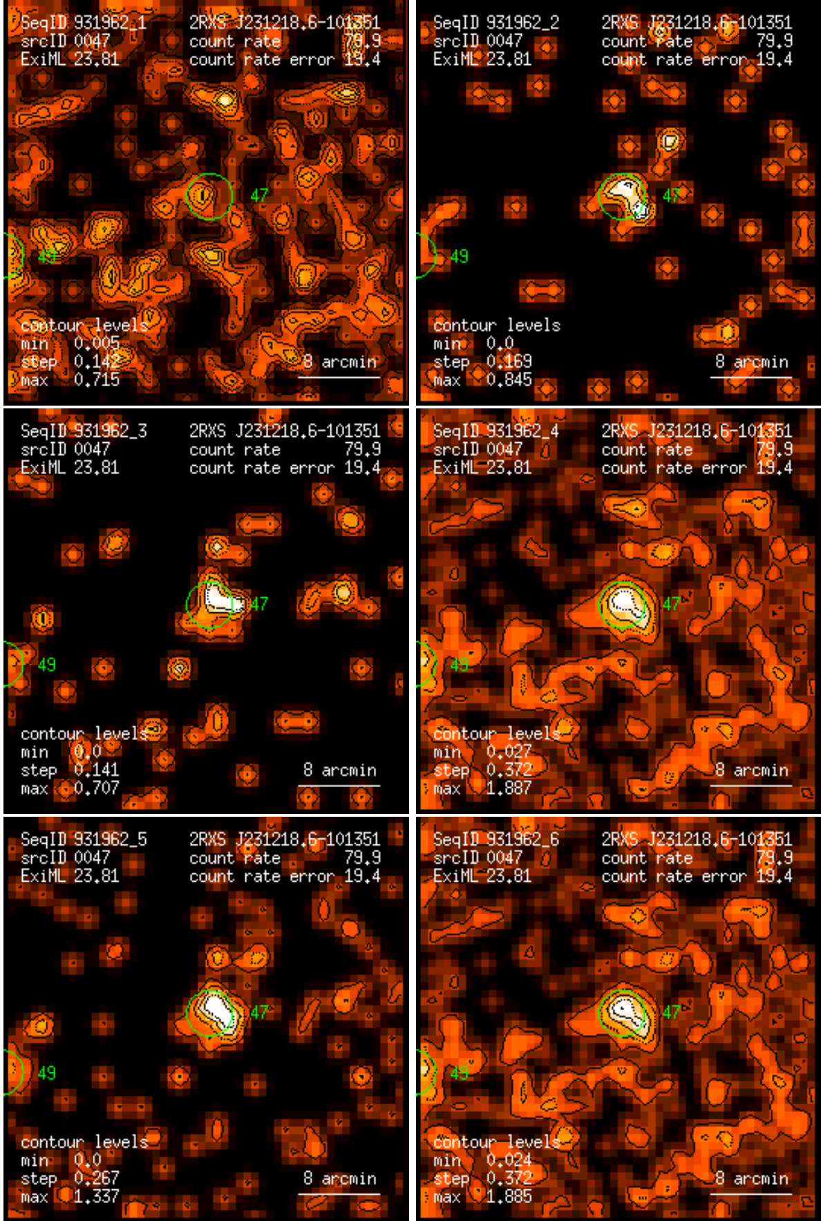
Figure 47: RASS 931962: detection 0047: band rate images, Gaussian filter: (1) PSPC channels 11 – 41, (2) 52 – 90, (3) 91 – 201, (4) 11 – 235, (5) 52 – 201, (6) 11 – 201. Broad band rates in counts/ks. Band rate contour levels in counts/ks/arcmin 2 .
