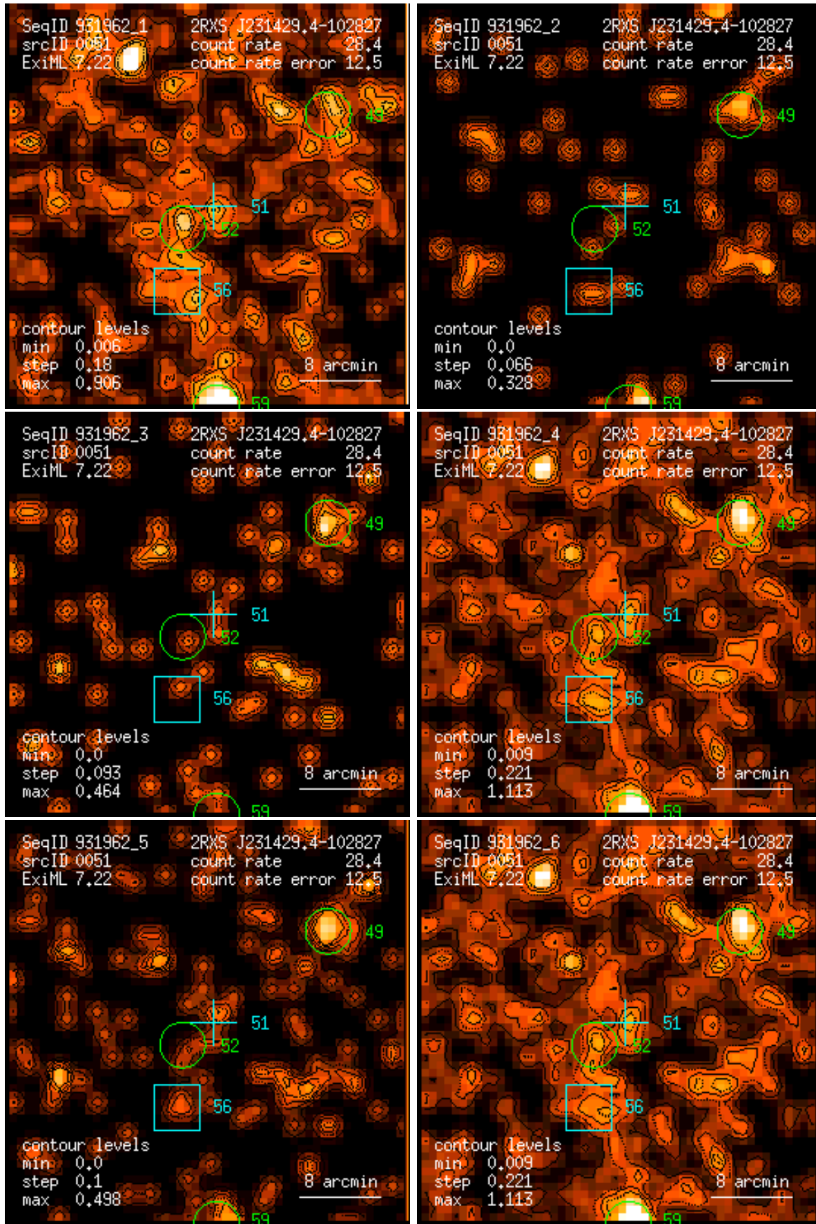
Figure 51: RASS 931962: detection 0051: band rate images, Gaussian filter: (1) PSPP channels 11 – 41, (2) 52 – 90, (3) 91 – 201, (4) 11 – 235, (5) 52 – 201, (6) 11 – 201. Broad band rates in counts/ks. Band rate contour levels in counts/ks/arcmin 2 .
