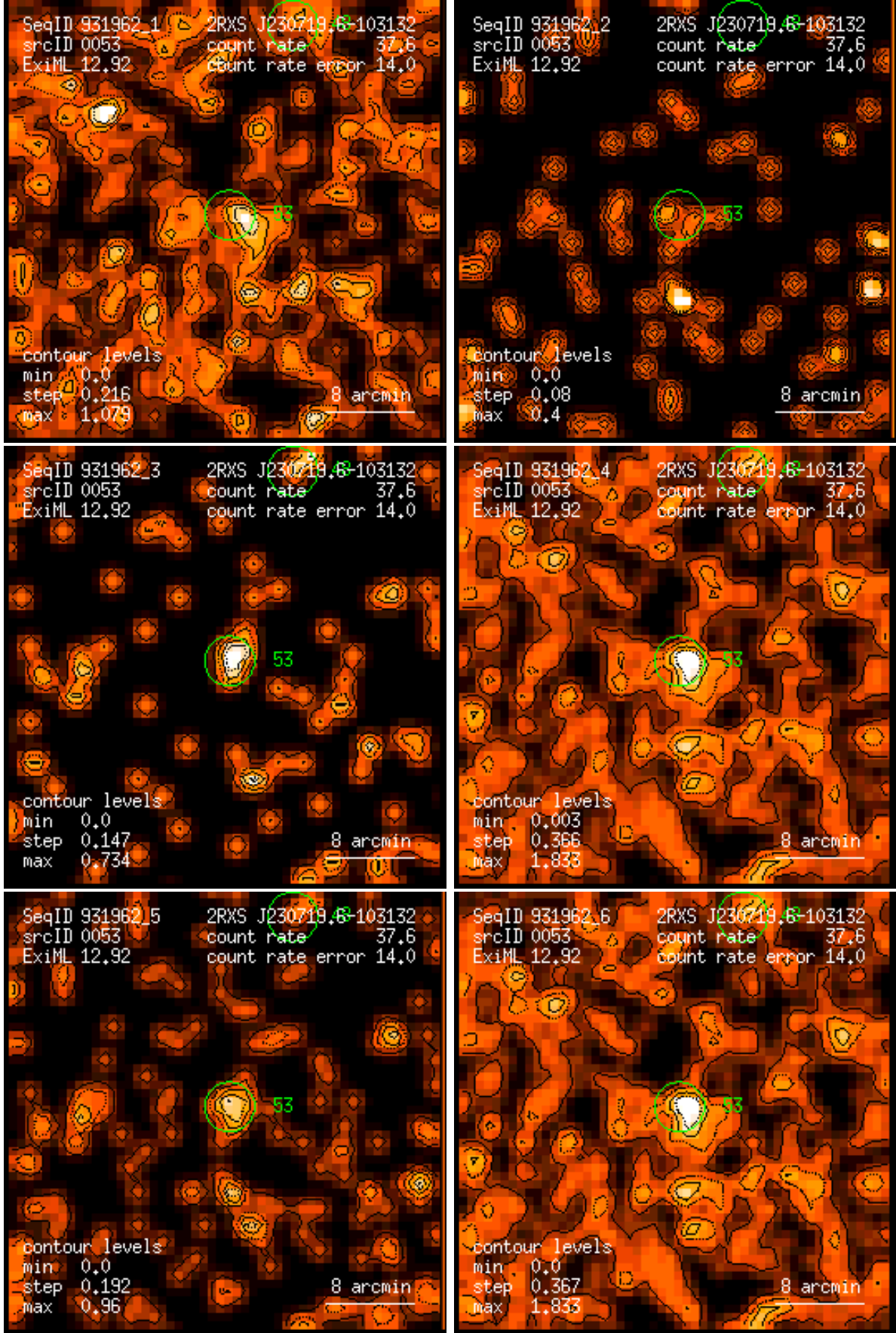
Figure 53: RASS 931962: detection 0053: band rate images, Gaussian filter: (1) PSPC channels 11 – 41, (2) 52 – 90, (3) 91 – 201, (4) 11 – 235, (5) 52 – 201, (6) 11 – 201. Broad band rates in counts/ks. Band rate contour levels in counts/ks/arcmin 2 .
