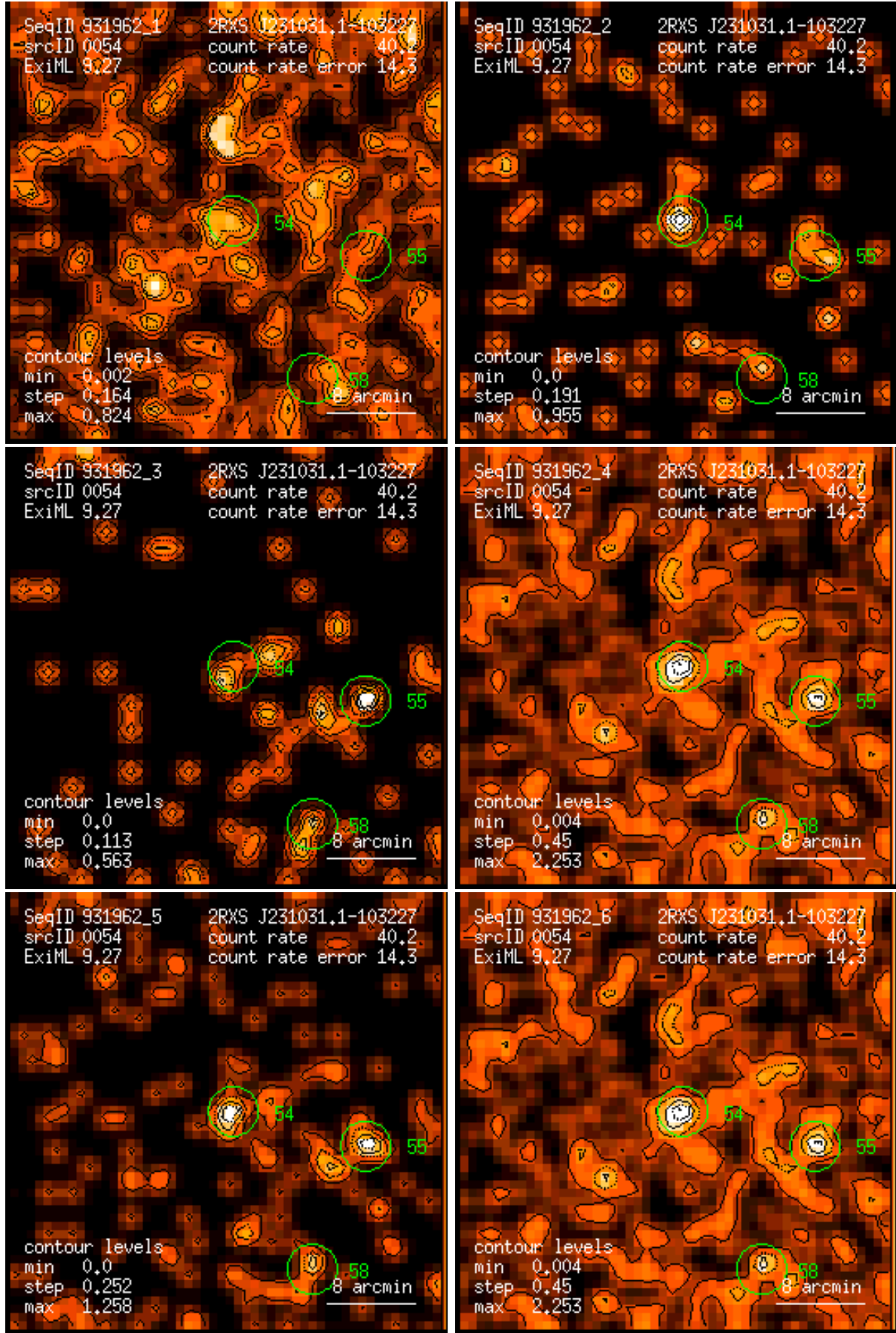
Figure 54: RASS 931962: detection 0054: band rate images, Gaussian filter: (1) PSPC channels 11 – 41, (2) 52 – 90, (3) 91 – 201, (4) 11 – 235, (5) 52 – 201, (6) 11 – 201. Broad band rates in counts/ks. Band rate contour levels in counts/ks/arcmin 2 .
