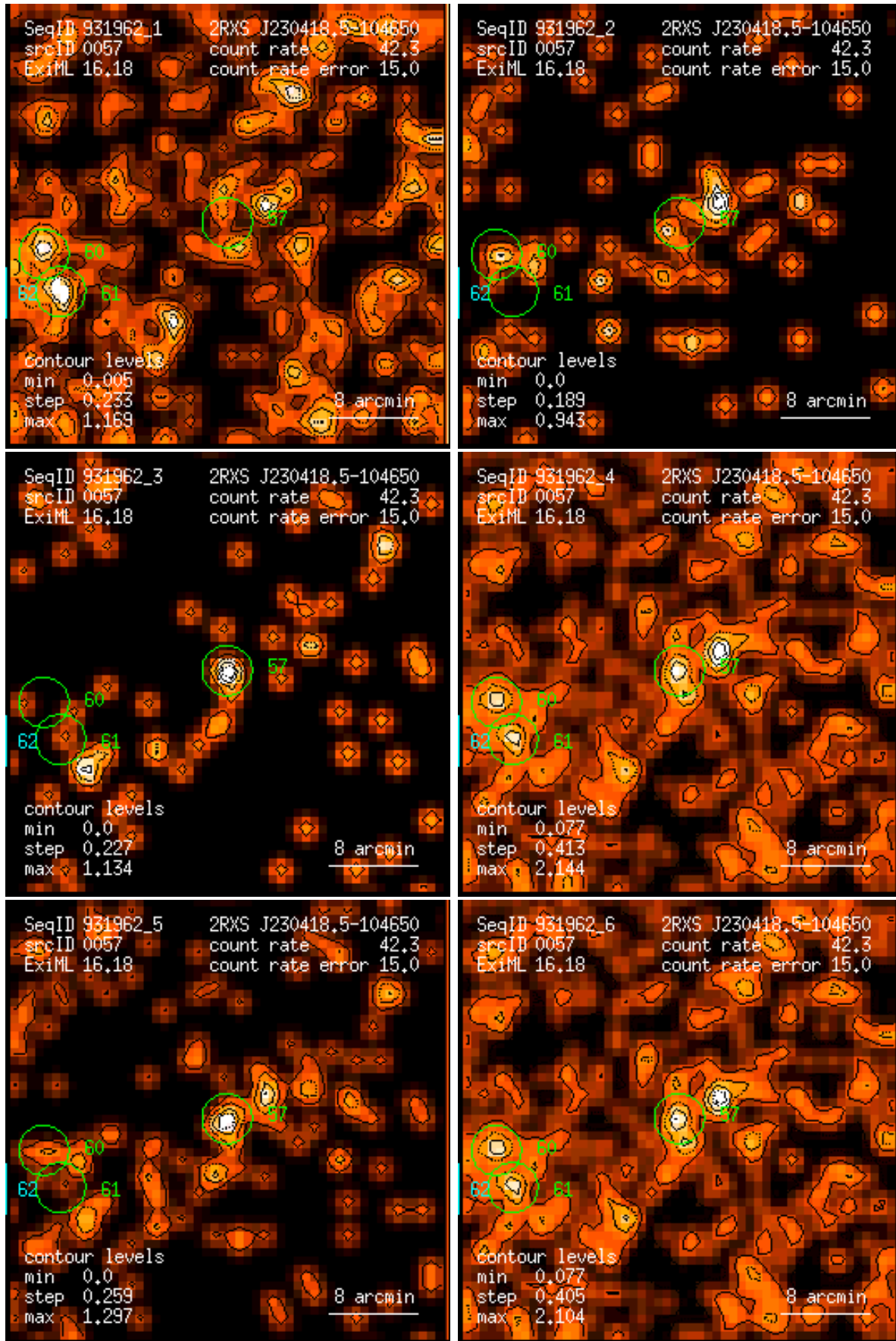
Figure 57: RASS 931962: detection 0057: band rate images, Gaussian filter: (1) PSPC channels 11 – 41, (2) 52 – 90, (3) 91 – 201, (4) 11 – 235, (5) 52 – 201, (6) 11 – 201. Broad band rates in counts/ks. Band rate contour levels in counts/ks/arcmin 2 .
