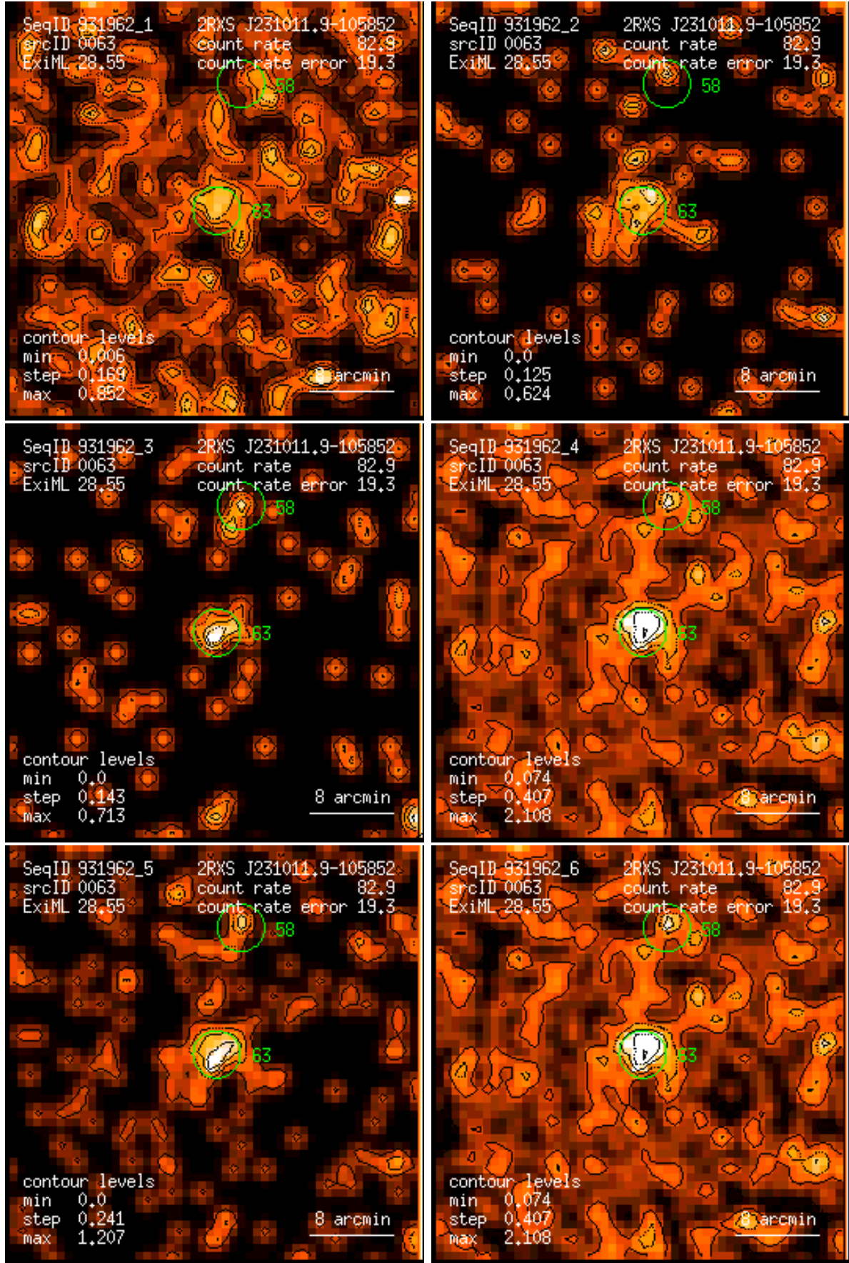
Figure 63: RASS 931962: detection 0063: band rate images, Gaussian filter: (1) PSPC channels 11 – 41, (2) 52 – 90, (3) 91 – 201, (4) 11 – 235, (5) 52 – 201, (6) 11 – 201. Broad band rates in counts/ks. Band rate contour levels in counts/ks/arcmin 2 .
