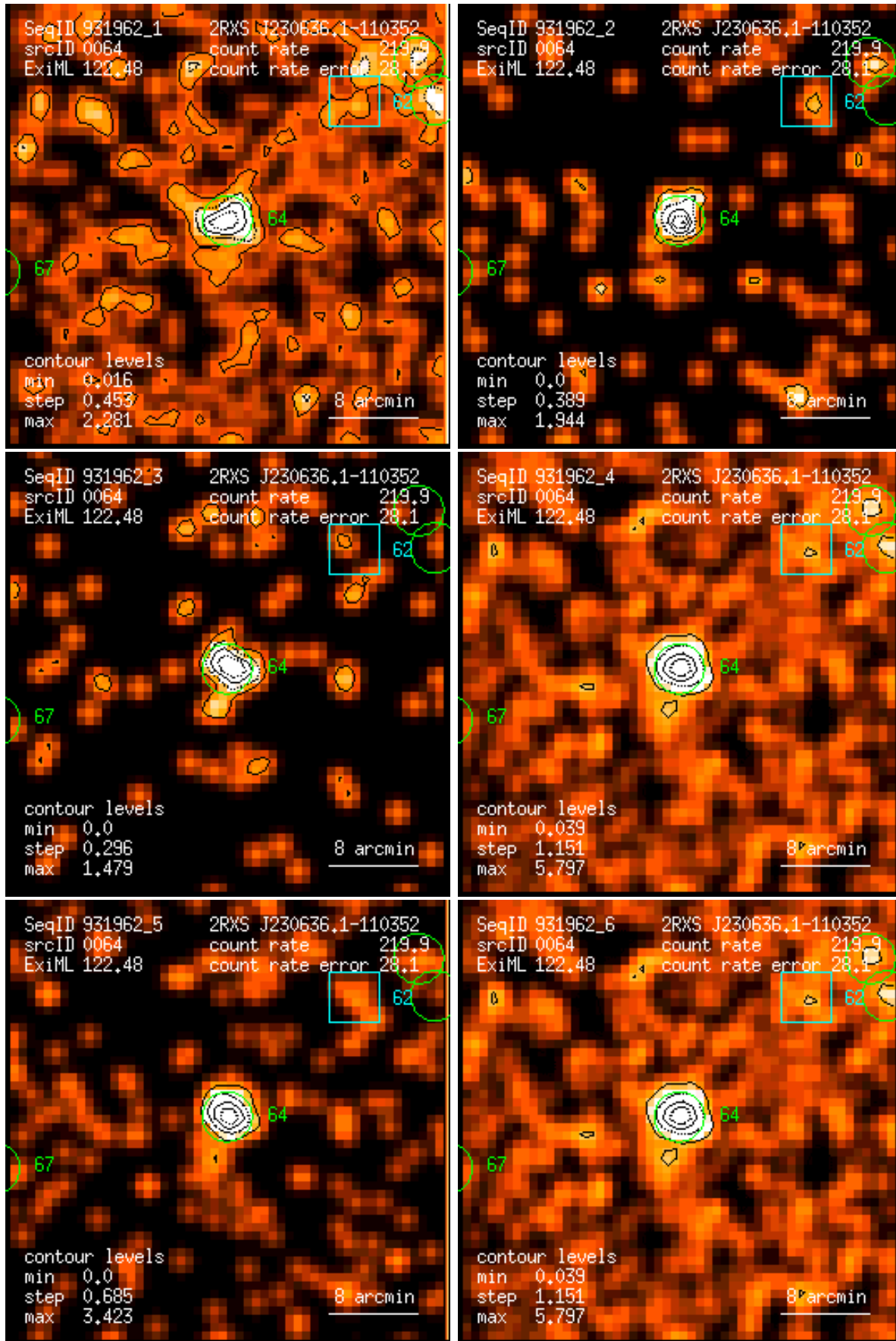
Figure 64: RASS 931962: detection 0064: band rate images, Gaussian filter: (1) PSPC channels 11 – 41, (2) 52 – 90, (3) 91 – 201, (4) 11 – 235, (5) 52 – 201, (6) 11 – 201. Broad band rates in counts/ks. Band rate contour levels in counts/ks/arcmin 2 .
