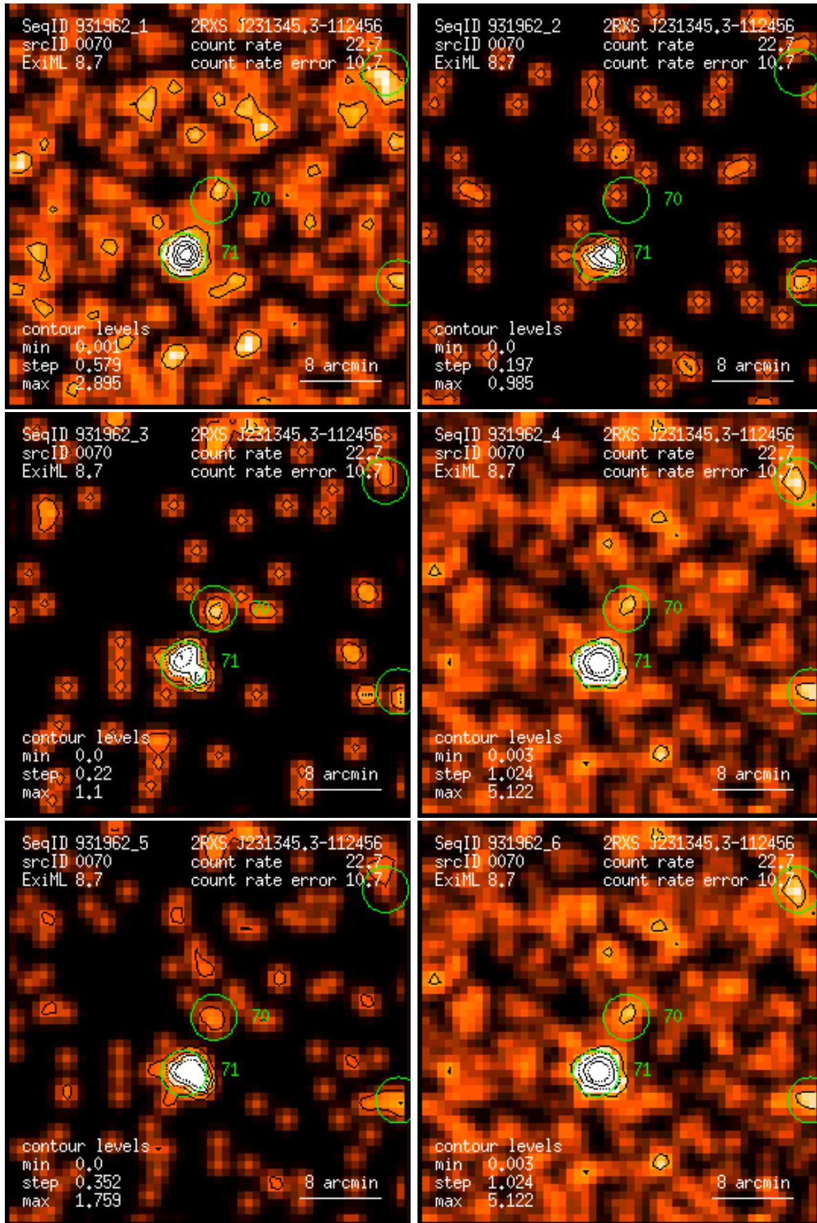
Figure 70: RASS 931962: detection 0070: band rate images, Gaussian filter: (1) PSPC channels 11 – 41, (2) 52 – 90, (3) 91 – 201, (4) 11 – 235, (5) 52 – 201, (6) 11 – 201. Broad band rates in counts/ks. Band rate contour levels in counts/ks/arcmin 2 .
