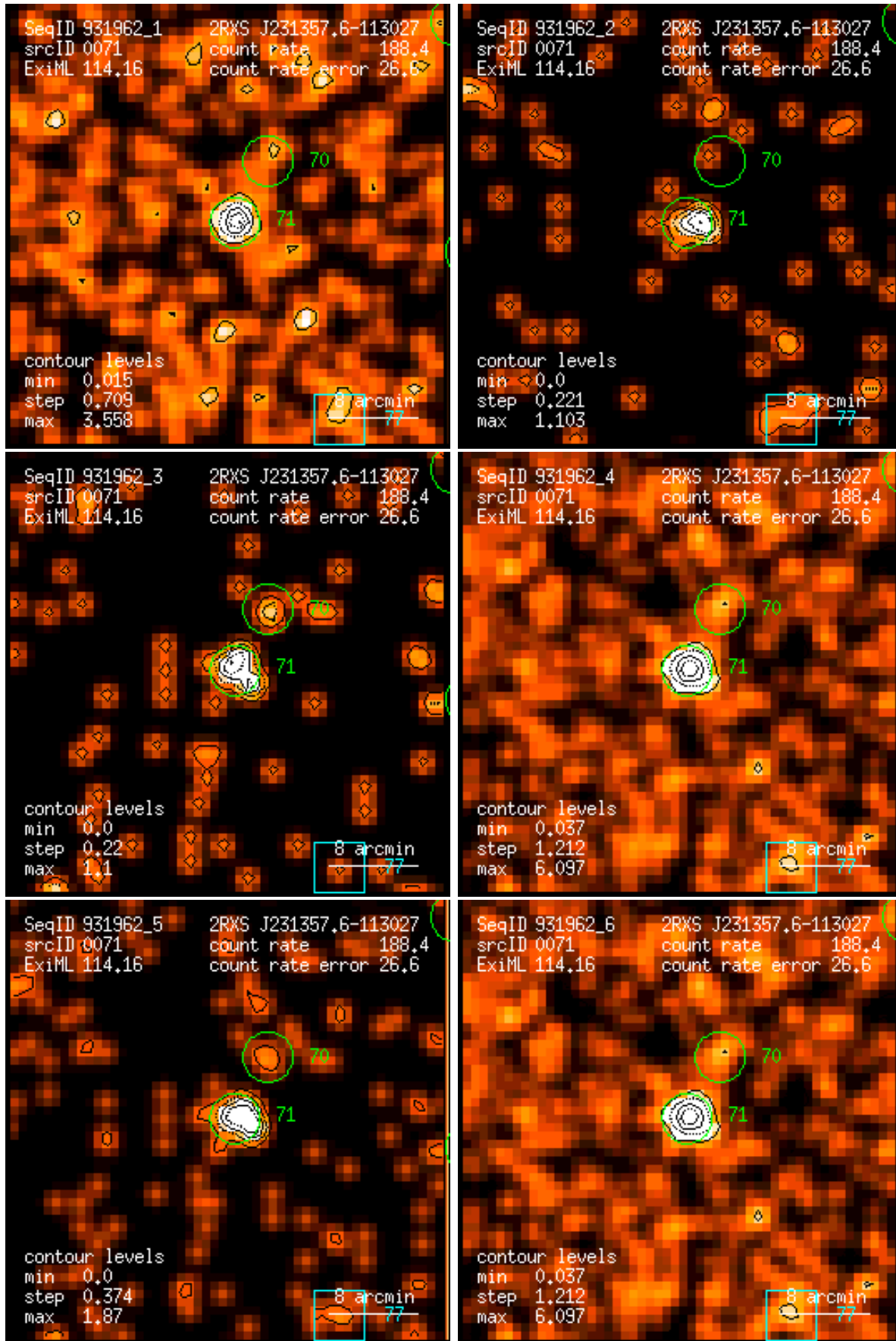
Figure 71: RASS 931962: detection 0071: band rate images, Gaussian filter: (1) PSPC channels 11 – 41, (2) 52 – 90, (3) 91 – 201, (4) 11 – 235, (5) 52 – 201, (6) 11 – 201. Broad band rates in counts/ks. Band rate contour levels in counts/ks/arcmin 2 .
