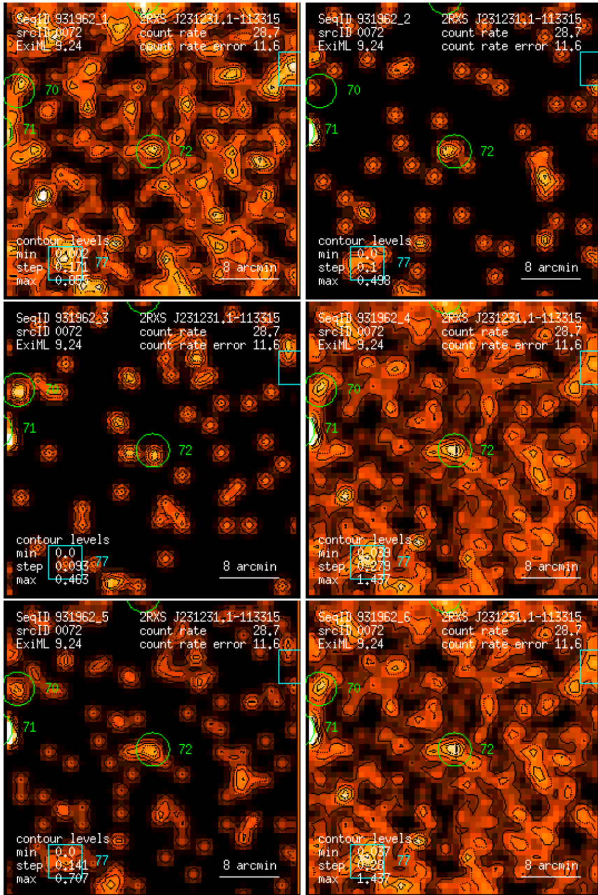
Figure 72: RASS 931962: detection 0072: band rate images, Gaussian filter: (1) PSPC channels 11 – 41, (2) 52 – 90, (3) 91 – 201, (4) 11 – 235, (5) 52 – 201, (6) 11 – 201. Broad band rates in counts/ks. Band rate contour levels in counts/ks/arcmin 2 .
