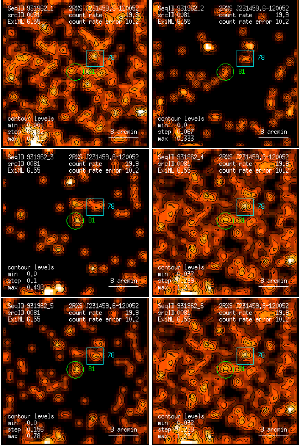
Figure 81: RASS 931962: detection 0081: band rate images, Gaussian filter: (1) PSPC channels 11 – 41, (2) 52 – 90, (3) 91 – 201, (4) 11 – 235, (5) 52 – 201, (6) 11 – 201. Broad band rates in counts/ks. Band rate contour levels in counts/ks/arcmin 2 .
