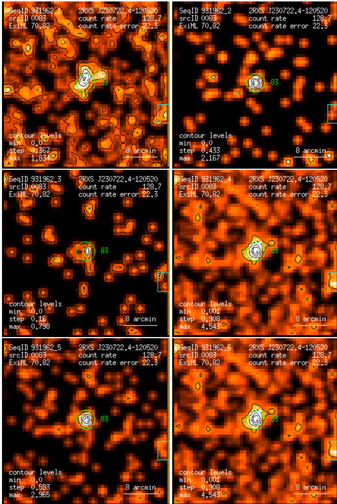
Figure 83: RASS 931962: detection 0083: band rate images, Gaussian filter: (1) PSPC channels 11 – 41, (2) 52 – 90, (3) 91 – 201, (4) 11 – 235, (5) 52 – 201, (6) 11 – 201. Broad band rates in counts/ks. Band rate contour levels in counts/ks/arcmin 2 .
