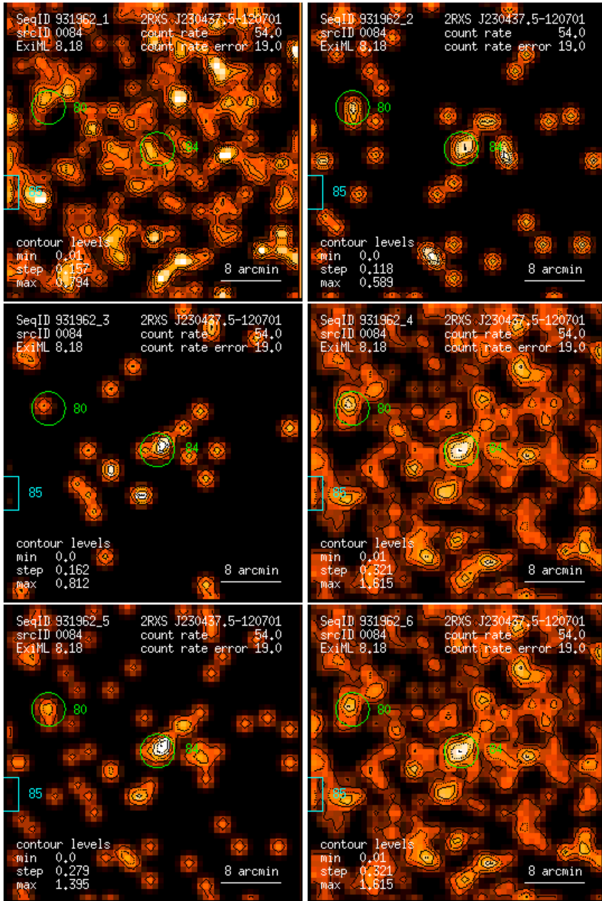
Figure 84: RASS 931962: detection 0084: band rate images, Gaussian filter: (1) PSPC channels 11 – 41, (2) 52 – 90, (3) 91 – 201, (4) 11 – 235, (5) 52 – 201, (6) 11 – 201. Broad band rates in counts/ks. Band rate contour levels in counts/ks/arcmin 2 .
