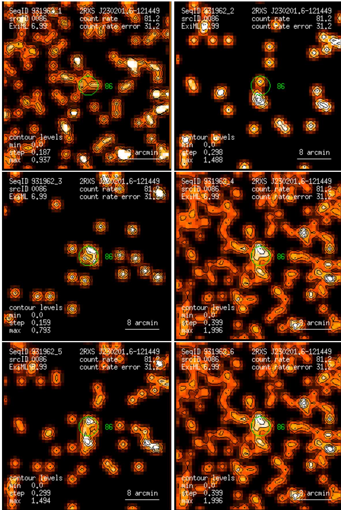
Figure 86: RASS 931962: detection 0086: band rate images, Gaussian filter: (1) PSPC channels 11 – 41, (2) 52 – 90, (3) 91 – 201, (4) 11 – 235, (5) 52 – 201, (6) 11 – 201. Broad band rates in counts/ks. Band rate contour levels in counts/ks/arcmin 2 .
