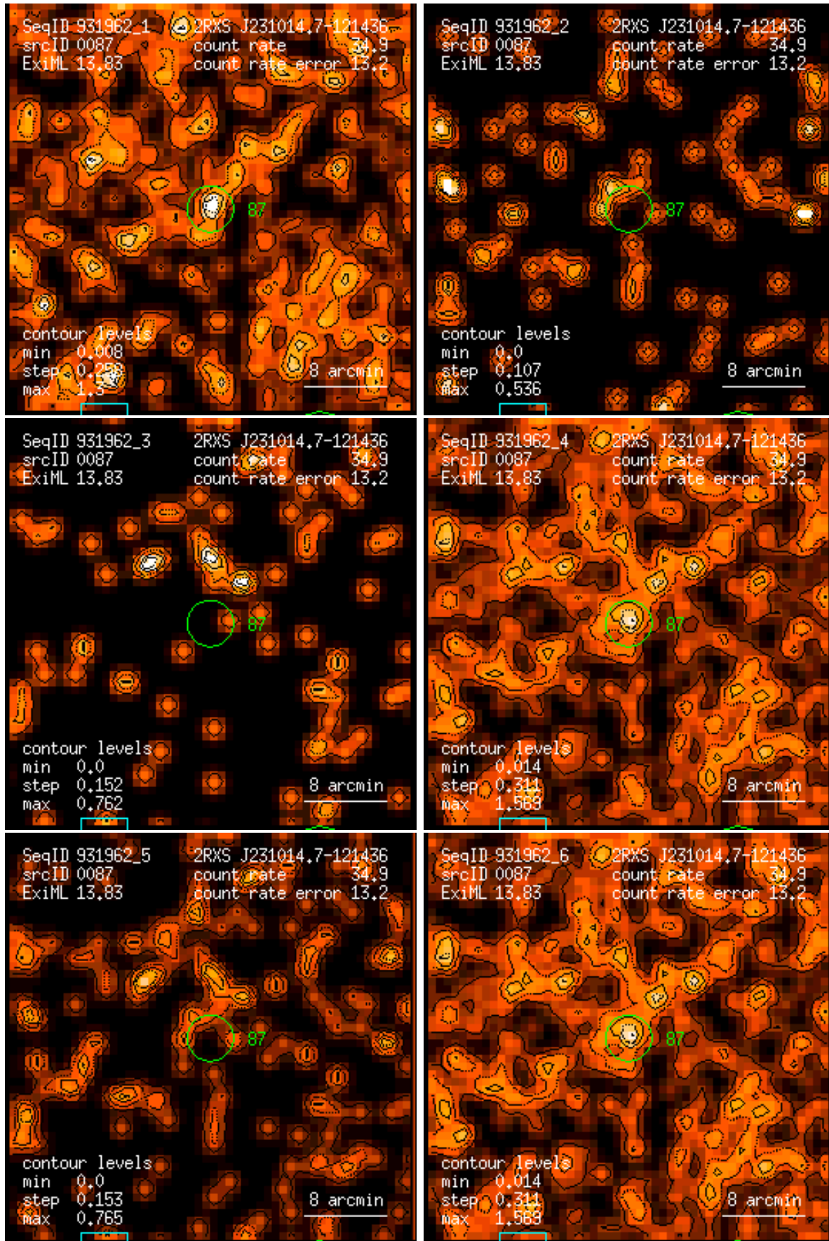
Figure 87: RASS 931962: detection 0087: band rate images, Gaussian filter: (1) PSPC channels 11 – 41, (2) 52 – 90, (3) 91 – 201, (4) 11 – 235, (5) 52 – 201, (6) 11 – 201. Broad band rates in counts/ks. Band rate contour levels in counts/ks/arcmin 2 .
