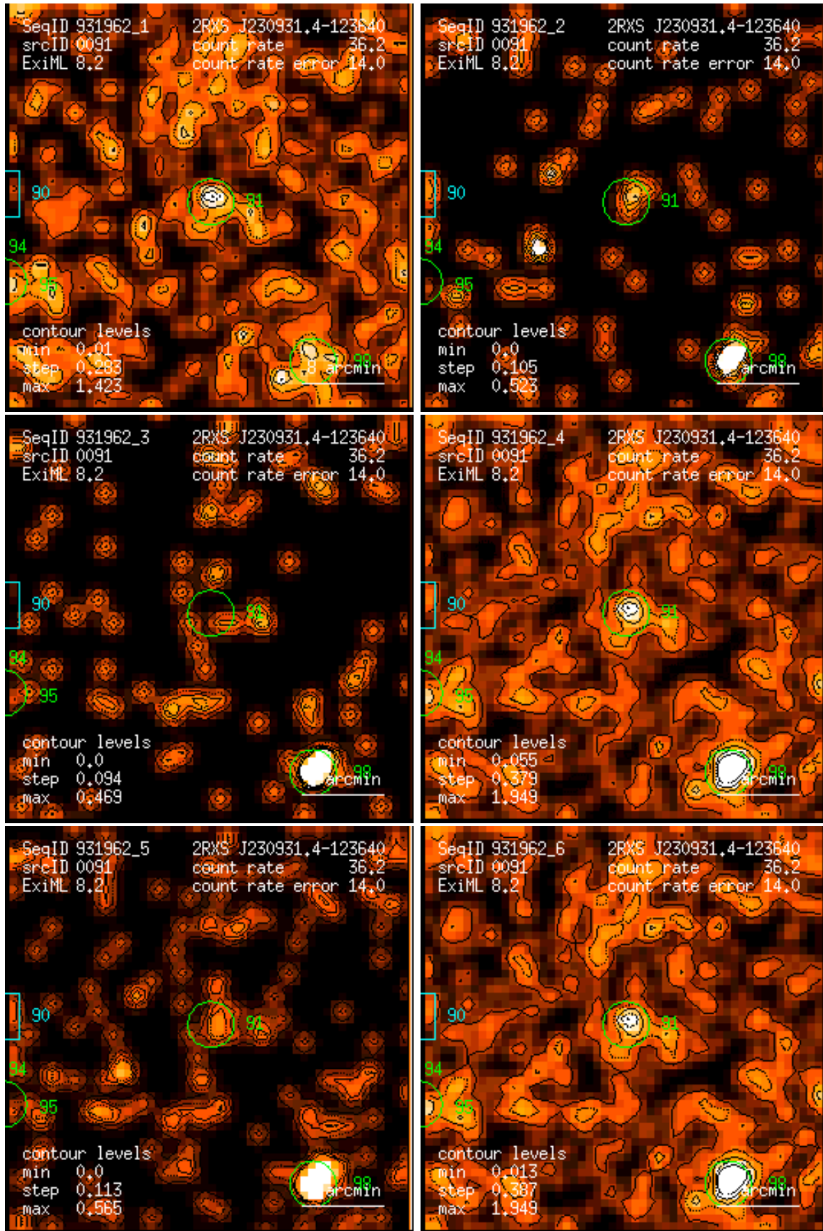
Figure 91: RASS 931962: detection 0091: band rate images, Gaussian filter: (1) PSPC channels 11 – 41, (2) 52 – 90, (3) 91 – 201, (4) 11 – 235, (5) 52 – 201, (6) 11 – 201. Broad band rates in counts/ks. Band rate contour levels in counts/ks/arcmin 2 .
