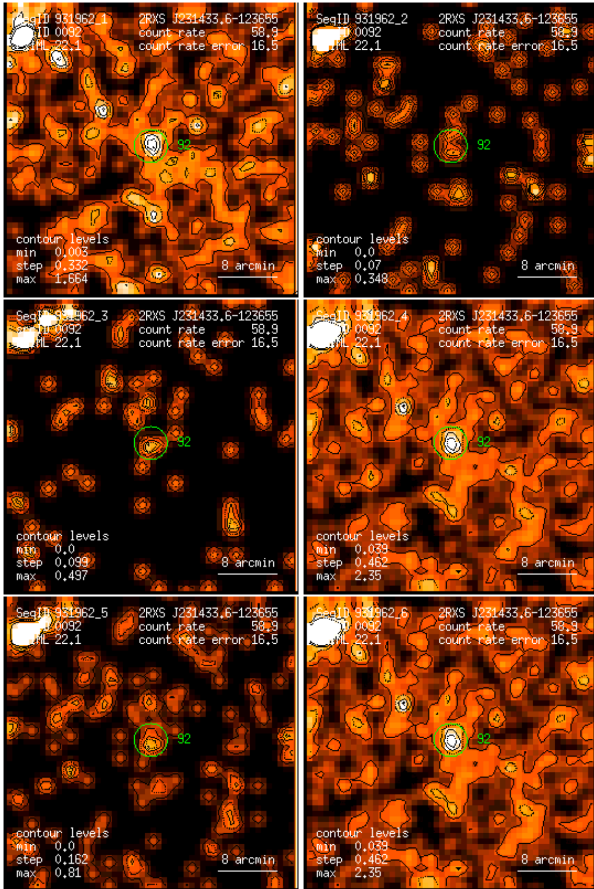
Figure 92: RASS 931962: detection 0092: band rate images, Gaussian filter: (1) PSPC channels 11 – 41, (2) 52 – 90, (3) 91 – 201, (4) 11 – 235, (5) 52 – 201, (6) 11 – 201. Broad band rates in counts/ks. Band rate contour levels in counts/ks/arcmin 2 .
