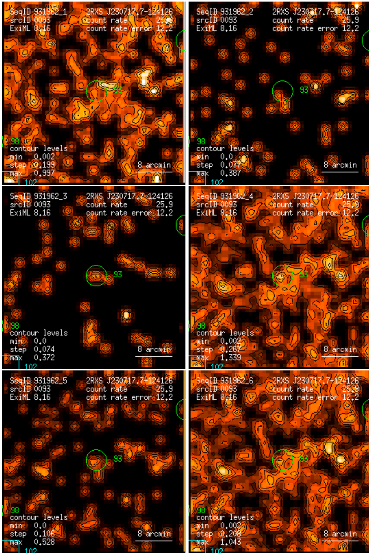
Figure 93: RASS 931962: detection 0093: band rate images, Gaussian filter: (1) PSPC channels 11 – 41, (2) 52 – 90, (3) 91 – 201, (4) 11 – 235, (5) 52 – 201, (6) 11 – 201. Broad band rates in counts/ks. Band rate contour levels in counts/ks/arcmin 2 .
