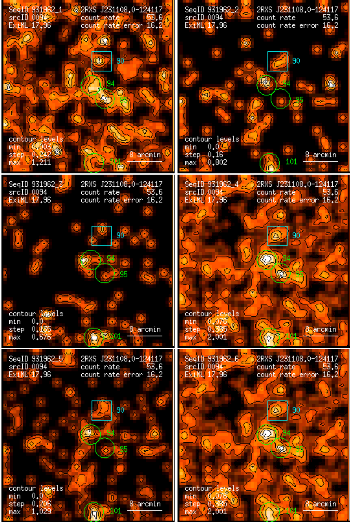
Figure 94: RASS 931962: detection 0094: band rate images, Gaussian filter: (1) PSPC channels 11 – 41, (2) 52 – 90, (3) 91 – 201, (4) 11 – 235, (5) 52 – 201, (6) 11 – 201. Broad band rates in counts/ks. Band rate contour levels in counts/ks/arcmin 2 .
