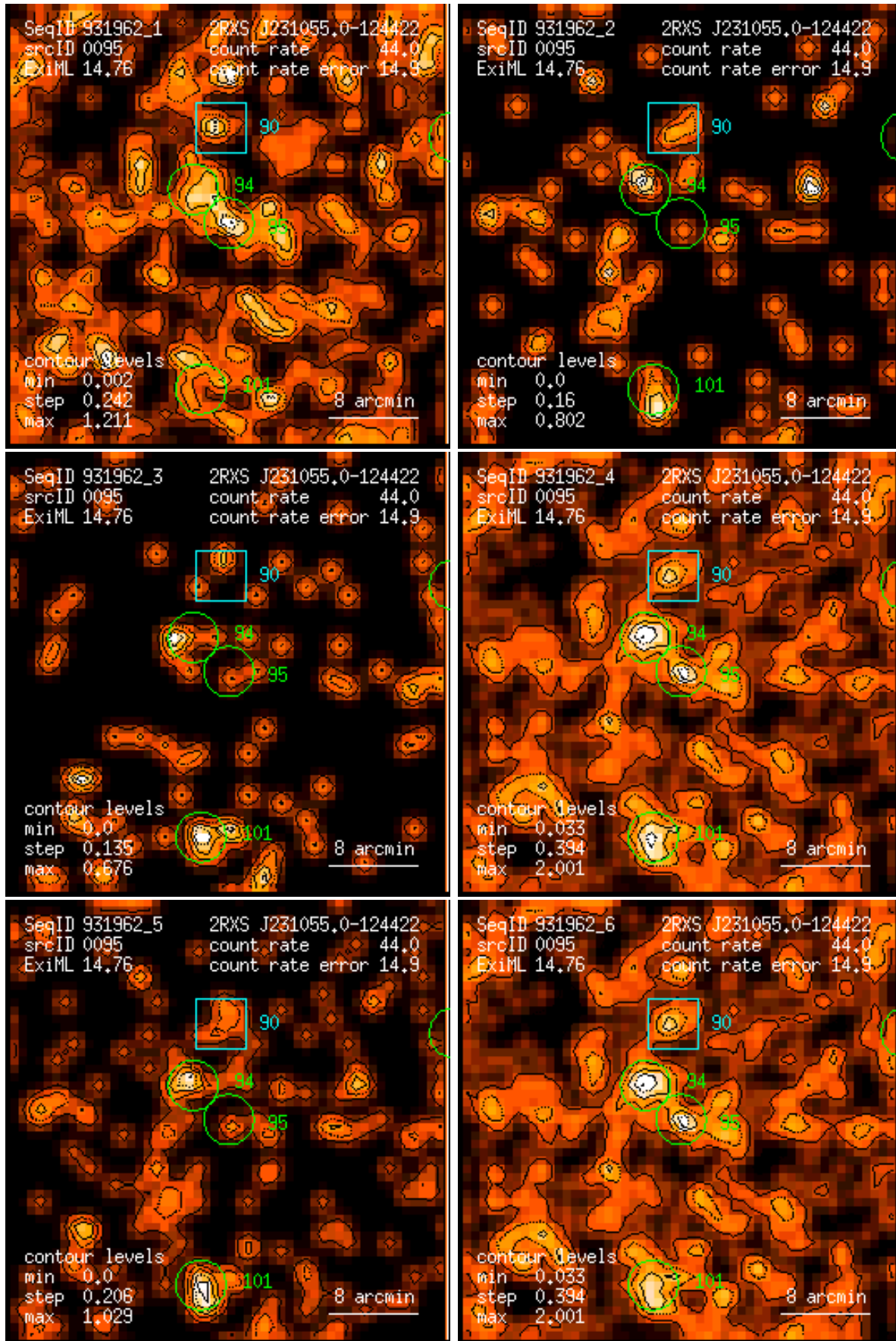
Figure 95: RASS 931962: detection 0095: band rate images, Gaussian filter: (1) PSPC channels 11 – 41, (2) 52 – 90, (3) 91 – 201, (4) 11 – 235, (5) 52 – 201, (6) 11 – 201. Broad band rates in counts/ks. Band rate contour levels in counts/ks/arcmin 2 .
