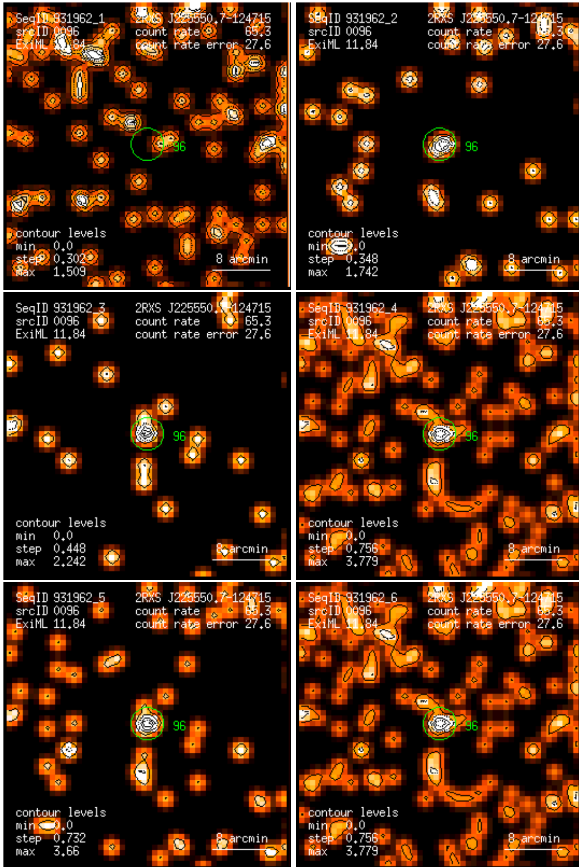
Figure 96: RASS 931962: detection 0096: band rate images, Gaussian filter: (1) PSPC channels 11 – 41, (2) 52 – 90, (3) 91 – 201, (4) 11 – 235, (5) 52 – 201, (6) 11 – 201. Broad band rates in counts/ks. Band rate contour levels in counts/ks/arcmin 2 .
