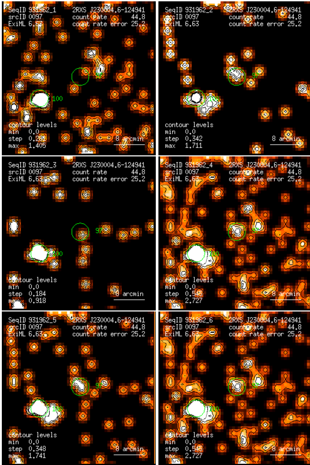
Figure 97: RASS 931962: detection 0097: band rate images, Gaussian filter: (1) PSPC channels 11 – 41, (2) 52 – 90, (3) 91 – 201, (4) 11 – 235, (5) 52 – 201, (6) 11 – 201. Broad band rates in counts/ks. Band rate contour levels in counts/ks/arcmin 2 .
