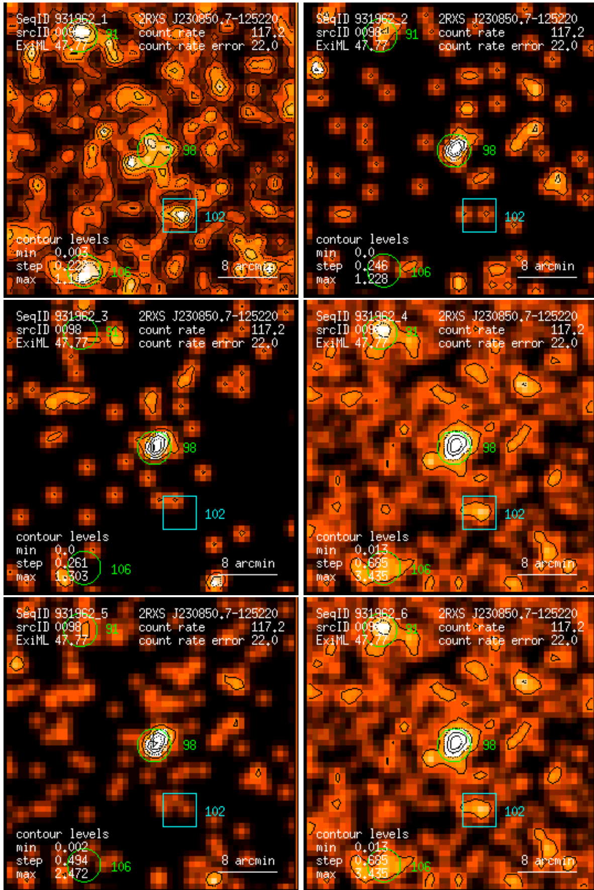
Figure 98: RASS 931962: detection 0098: band rate images, Gaussian filter: (1) PSPC channels 11 – 41, (2) 52 – 90, (3) 91 – 201, (4) 11 – 235, (5) 52 – 201, (6) 11 – 201. Broad band rates in counts/ks. Band rate contour levels in counts/ks/arcmin 2 .
