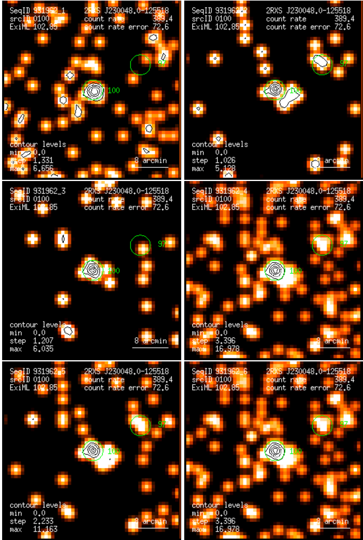
Figure 100: RASS 931962: detection 0100: band rate images, Gaussian filter: (1) PSPC channels 11 – 41, (2) 52 – 90, (3) 91 – 201, (4) 11 – 235, (5) 52 – 201, (6) 11 – 201. Broad band rates in counts/ks. Band rate contour levels in counts/ks/arcmin 2 .
