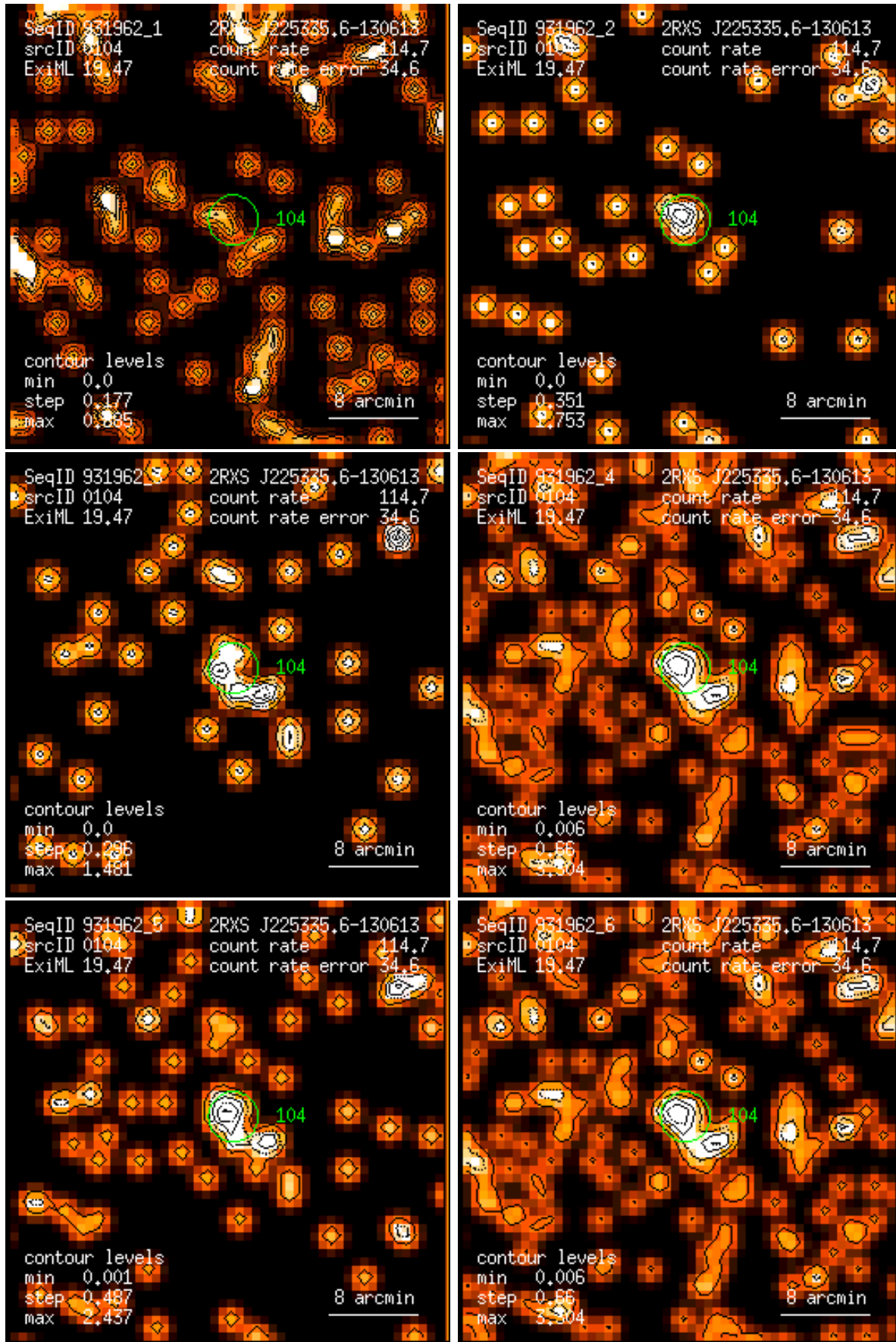
Figure 104: RASS 931962: detection 0104: band rate images, Gaussian filter: (1) PSPC channels 11 – 41, (2) 52 – 90, (3) 91 – 201, (4) 11 – 235, (5) 52 – 201, (6) 11 – 201. Broad band rates in counts/ks. Band rate contour levels in counts/ks/arcmin 2 .
