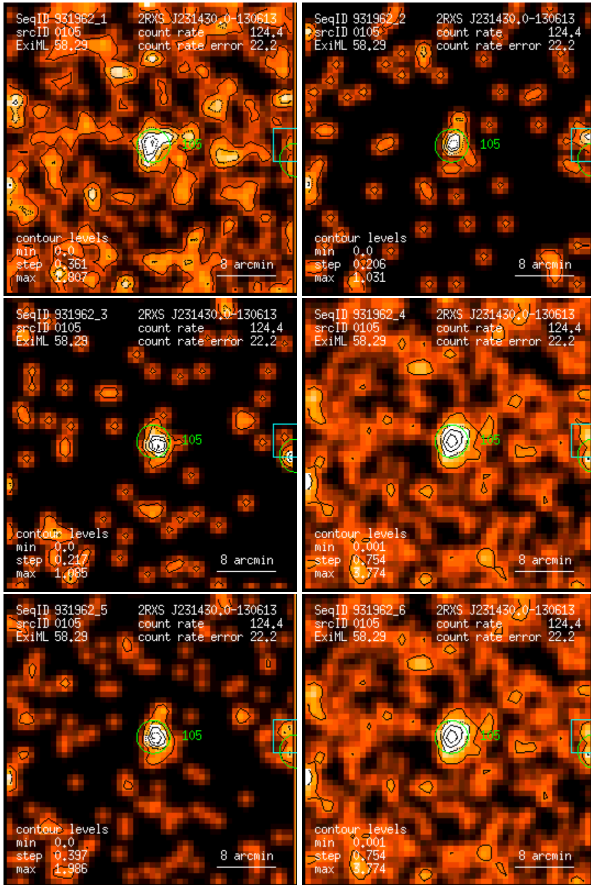
Figure 105: RASS 931962: detection 0105: band rate images, Gaussian filter: (1) PSPC channels 11 – 41, (2) 52 – 90, (3) 91 – 201, (4) 11 – 235, (5) 52 – 201, (6) 11 – 201. Broad band rates in counts/ks. Band rate contour levels in counts/ks/arcmin 2 .
